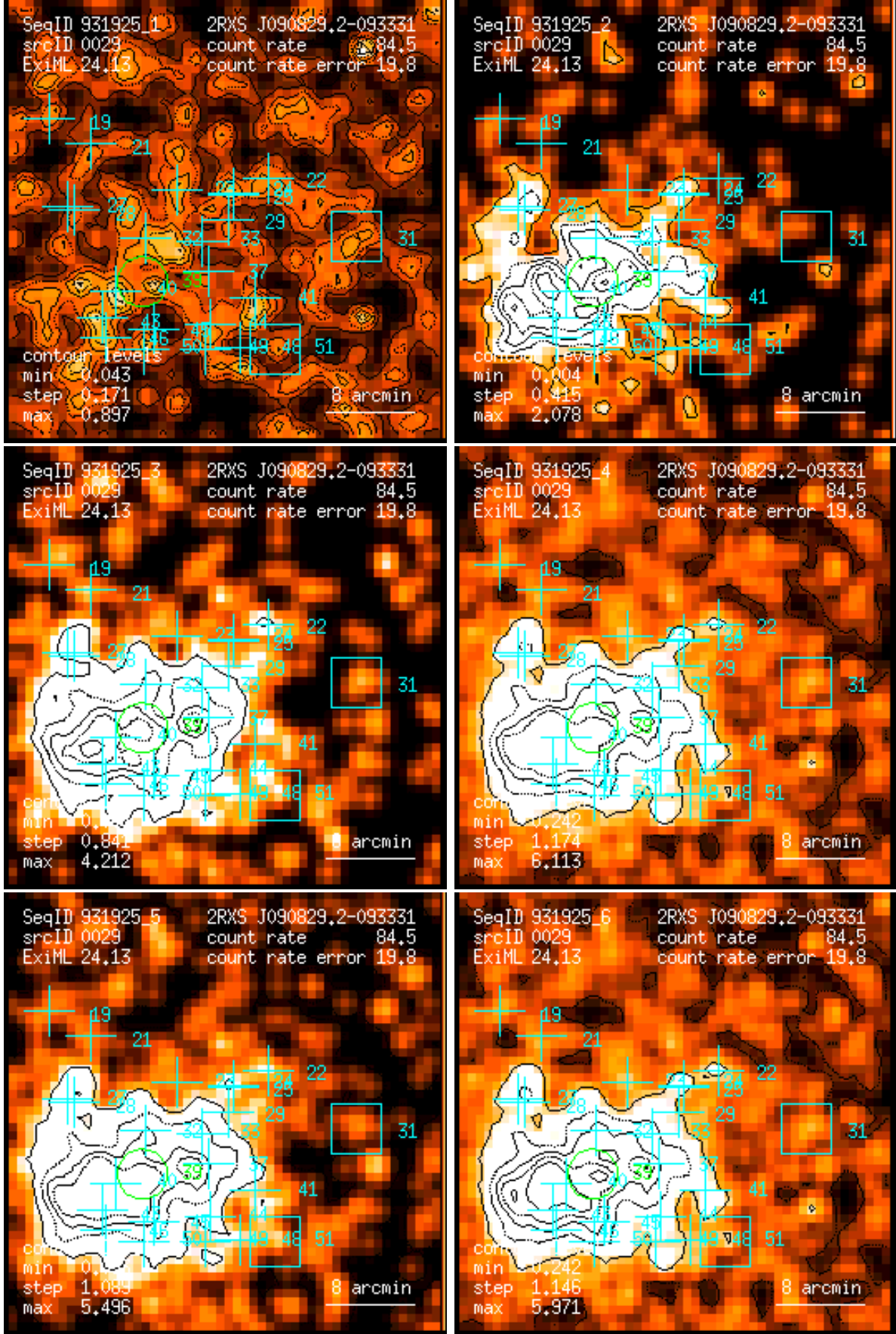
Figure 29: RASS 931925: detection 0029: band rate images, Gaussian filter: (1) PSPC channels 11 – 41, (2) 52 – 90, (3) 91 – 201, (4) 11 – 235, (5) 52 – 201, (6) 11 – 201. Broad band rates in counts/ks. Band rate contour levels in counts/ks/arcmin 2 .
