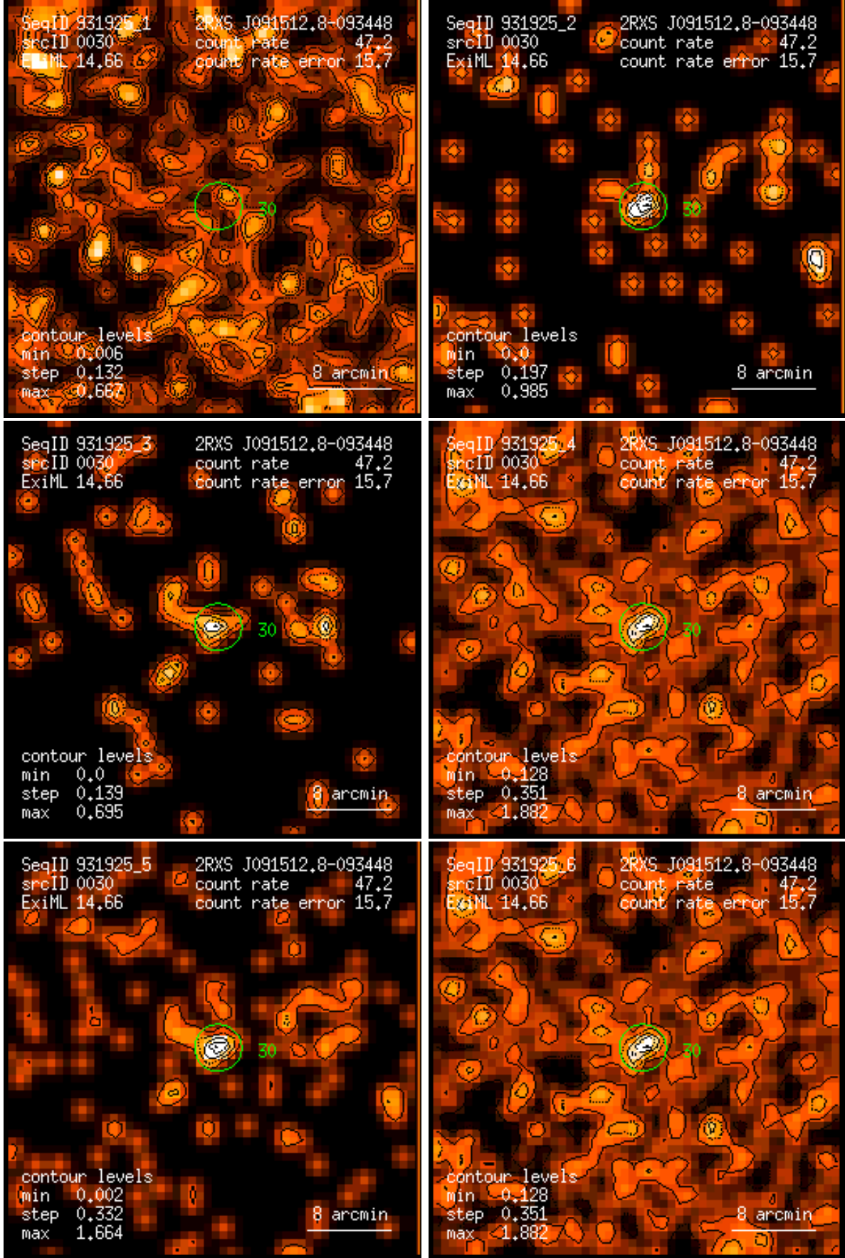
Figure 30: RASS 931925: detection 0030: band rate images, Gaussian filter: (1) PSPC channels 11 – 41, (2) 52 – 90, (3) 91 – 201, (4) 11 – 235, (5) 52 – 201, (6) 11 – 201. Broad band rates in counts/ks. Band rate contour levels in counts/ks/arcmin 2 .
