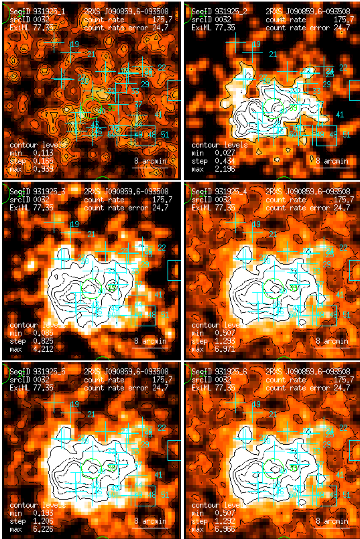
Figure 32: RASS 931925: detection 0032: band rate images, Gaussian filter: (1) PSPC channels 11 – 41, (2) 52 – 90, (3) 91 – 201, (4) 11 – 235, (5) 52 – 201, (6) 11 – 201. Broad band rates in counts/ks. Band rate contour levels in counts/ks/arcmin 2 .
