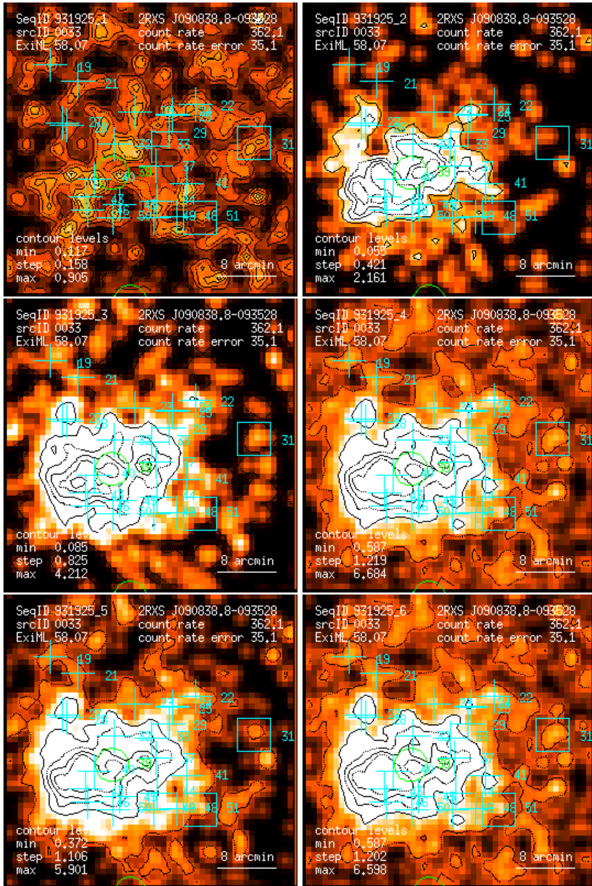
Figure 33: RASS 931925: detection 0033: band rate images, Gaussian filter: (1) PSPC channels 11 – 41, (2) 52 – 90, (3) 91 – 201, (4) 11 – 235, (5) 52 – 201, (6) 11 – 201. Broad band rates in counts/ks. Band rate contour levels in counts/ks/arcmin 2 .
