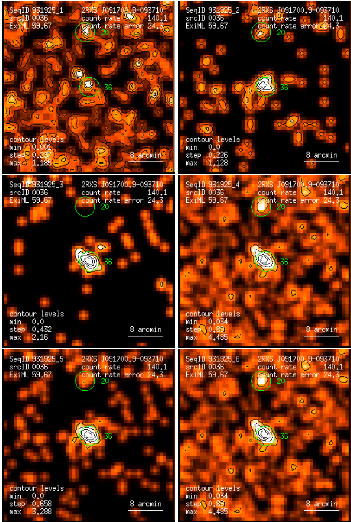
Figure 36: RASS 931925: detection 0036: band rate images, Gaussian filter: (1) PSPC channels 11 – 41, (2) 52 – 90, (3) 91 – 201, (4) 11 – 235, (5) 52 – 201, (6) 11 – 201. Broad band rates in counts/ks. Band rate contour levels in counts/ks/arcmin 2 .
