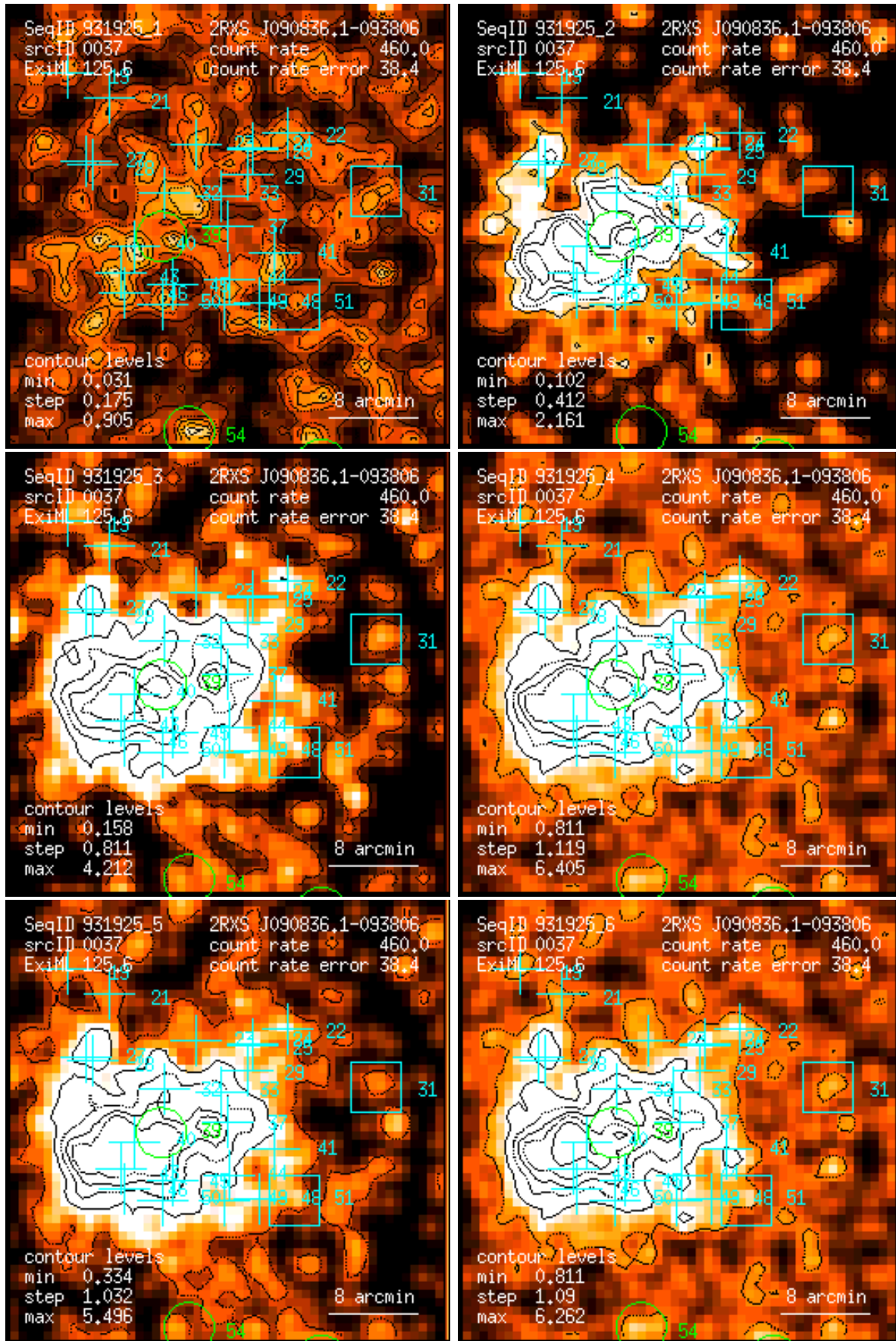
Figure 37: RASS 931925: detection 0037: band rate images, Gaussian filter: (1) PSPC channels 11 – 41, (2) 52 – 90, (3) 91 – 201, (4) 11 – 235, (5) 52 – 201, (6) 11 – 201. Broad band rates in counts/ks. Band rate contour levels in counts/ks/arcmin 2 .
