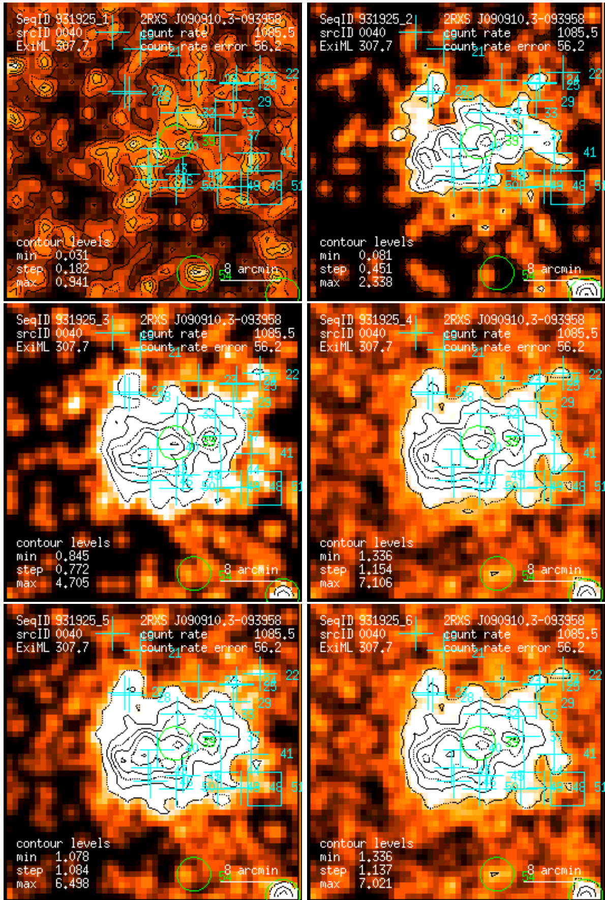
Figure 40: RASS 931925: detection 0040: band rate images, Gaussian filter: (1) PSPC channels 11 – 41, (2) 52 – 90, (3) 91 – 201, (4) 11 – 235, (5) 52 – 201, (6) 11 – 201. Broad band rates in counts/ks. Band rate contour levels in counts/ks/arcmin 2 .
