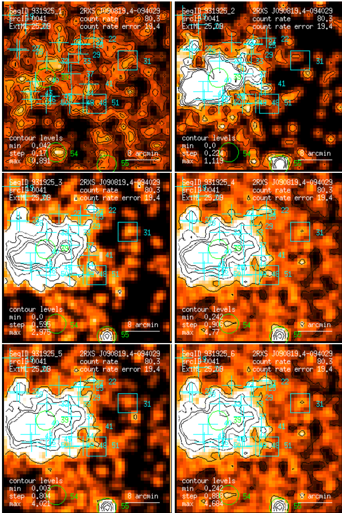
Figure 41: RASS 931925: detection 0041: band rate images, Gaussian filter: (1) PSPC channels 11 – 41, (2) 52 – 90, (3) 91 – 201, (4) 11 – 235, (5) 52 – 201, (6) 11 – 201. Broad band rates in counts/ks. Band rate contour levels in counts/ks/arcmin 2 .
