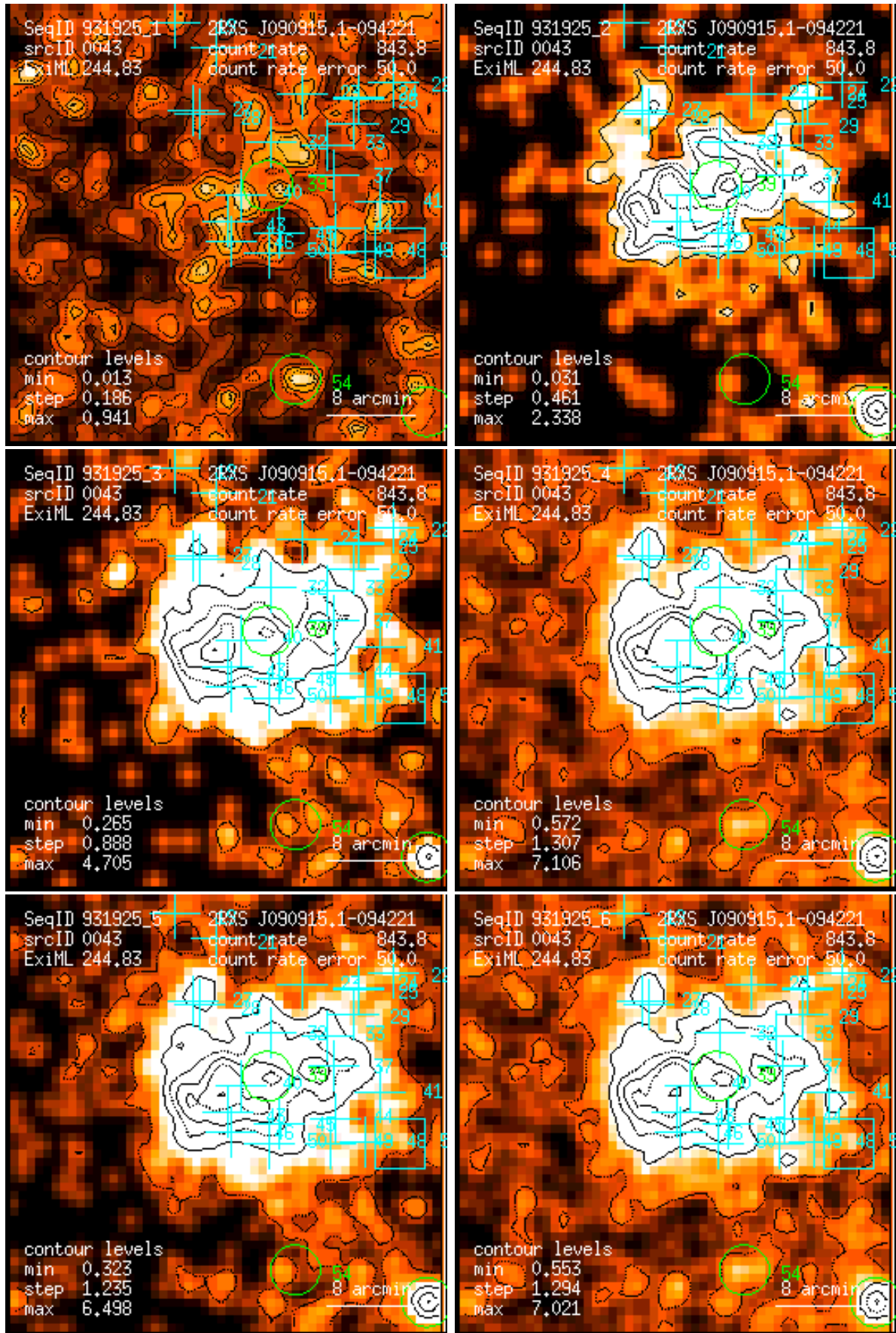
Figure 43: RASS 931925: detection 0043: band rate images, Gaussian filter: (1) PSPC channels 11 – 41, (2) 52 – 90, (3) 91 – 201, (4) 11 – 235, (5) 52 – 201, (6) 11 – 201. Broad band rates in counts/ks. Band rate contour levels in counts/ks/arcmin 2 .
