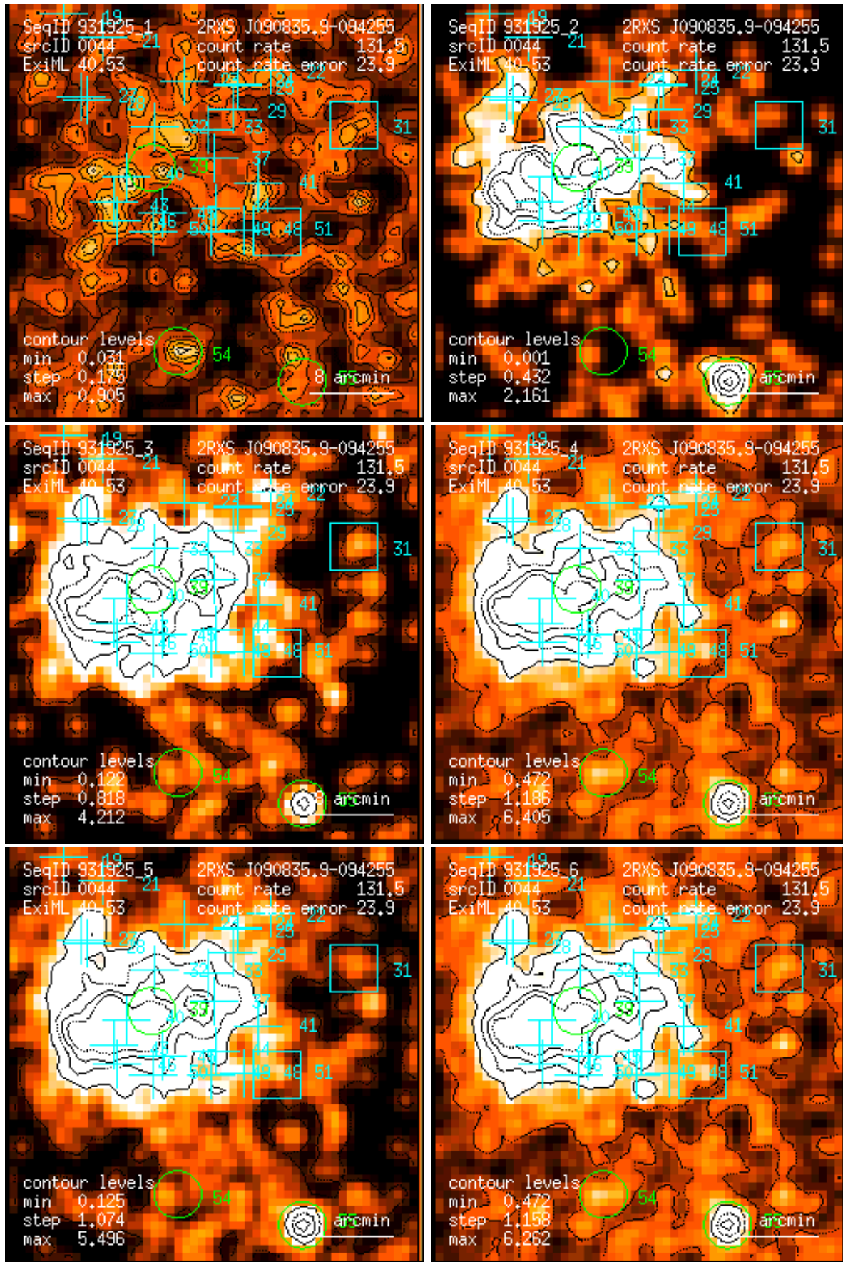
Figure 44: RASS 931925: detection 0044: band rate images, Gaussian filter: (1) PSPC channels 11 – 41, (2) 52 – 90, (3) 91 – 201, (4) 11 – 235, (5) 52 – 201, (6) 11 – 201. Broad band rates in counts/ks. Band rate contour levels in counts/ks/arcmin 2 .
