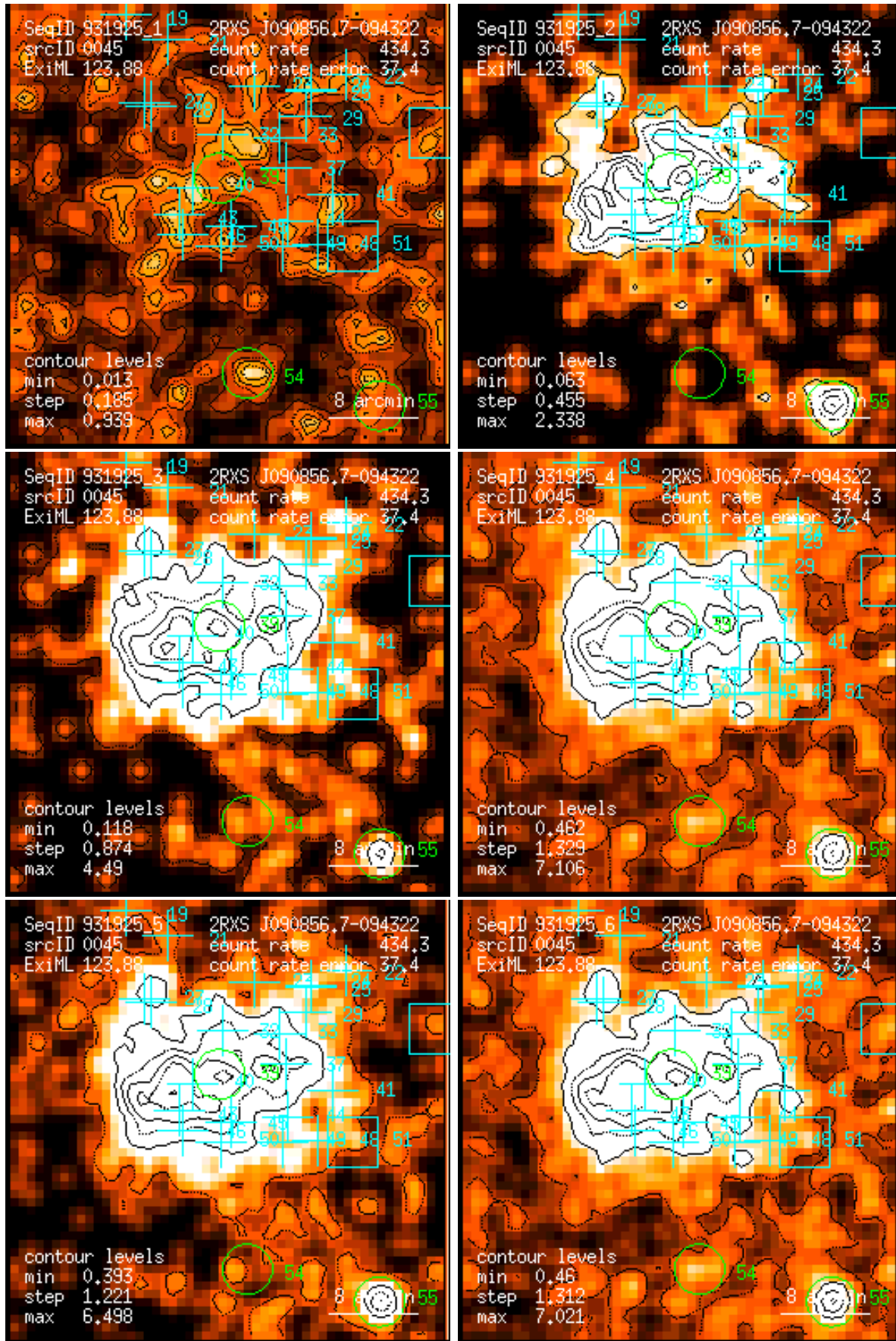
Figure 45: RASS 931925: detection 0045: band rate images, Gaussian filter: (1) PSPC channels 11 – 41, (2) 52 – 90, (3) 91 – 201, (4) 11 – 235, (5) 52 – 201, (6) 11 – 201. Broad band rates in counts/ks. Band rate contour levels in counts/ks/arcmin 2 .
