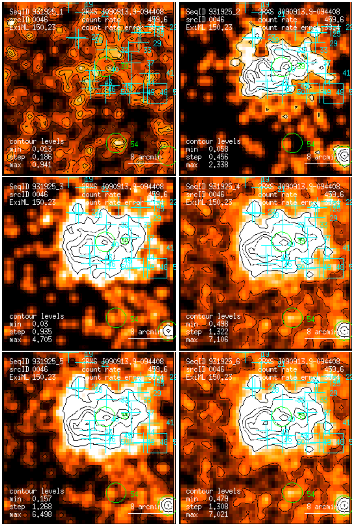
Figure 46: RASS 931925: detection 0046: band rate images, Gaussian filter: (1) PSPC channels 11 – 41, (2) 52 – 90, (3) 91 – 201, (4) 11 – 235, (5) 52 – 201, (6) 11 – 201. Broad band rates in counts/ks. Band rate contour levels in counts/ks/arcmin 2 .
