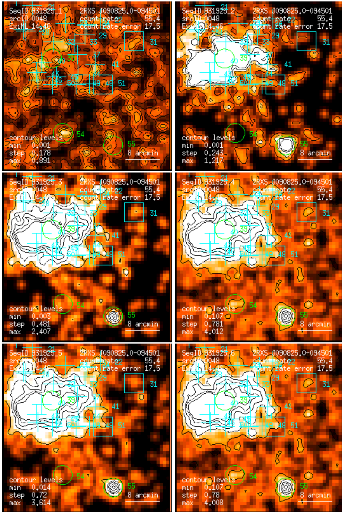
Figure 48: RASS 931925: detection 0048: band rate images, Gaussian filter: (1) PSPC channels 11 – 41, (2) 52 – 90, (3) 91 – 201, (4) 11 – 235, (5) 52 – 201, (6) 11 – 201. Broad band rates in counts/ks. Band rate contour levels in counts/ks/arcmin 2 .
