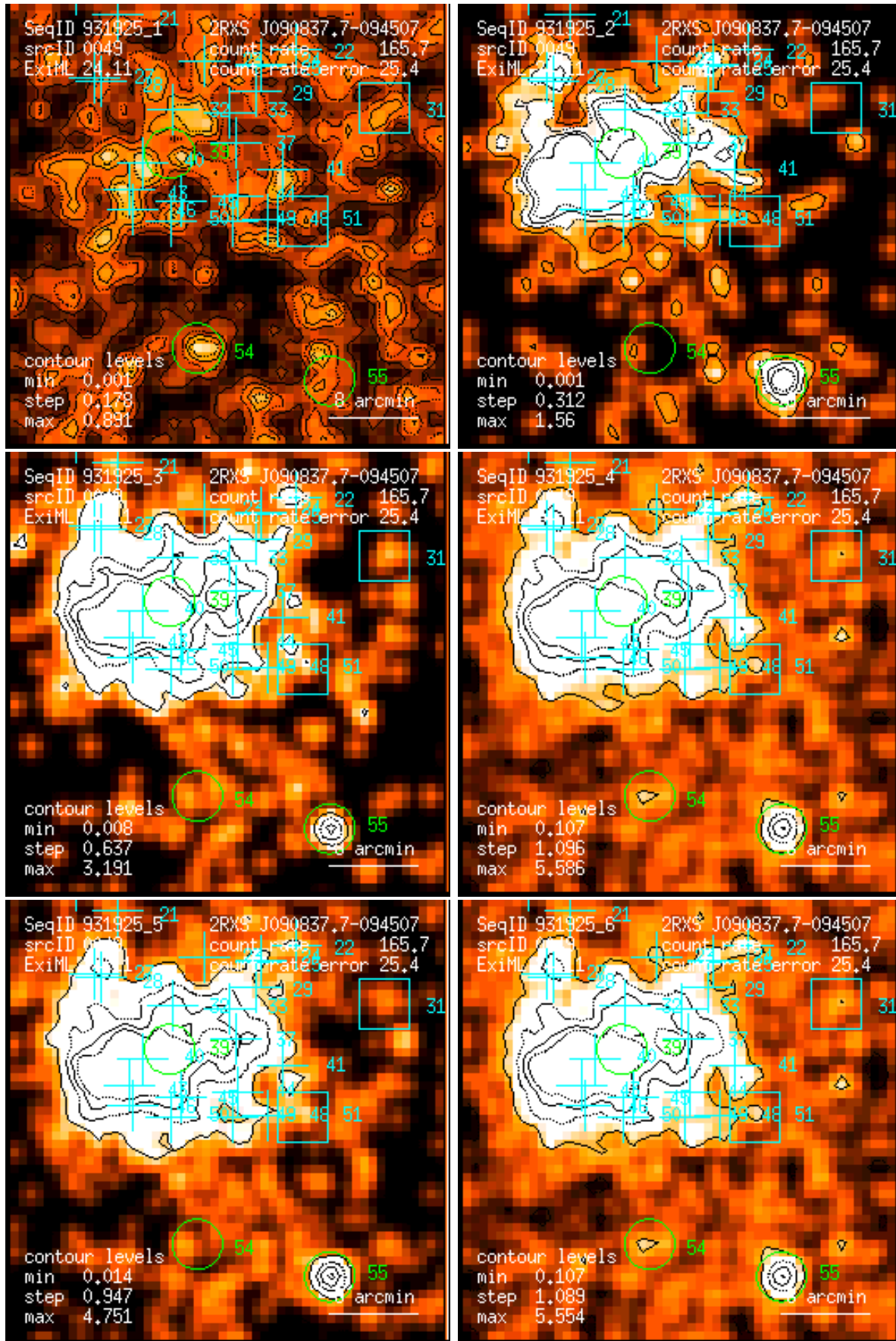
Figure 49: RASS 931925: detection 0049: band rate images, Gaussian filter: (1) PSPC channels 11 – 41, (2) 52 – 90, (3) 91 – 201, (4) 11 – 235, (5) 52 – 201, (6) 11 – 201. Broad band rates in counts/ks. Band rate contour levels in counts/ks/arcmin 2 .
