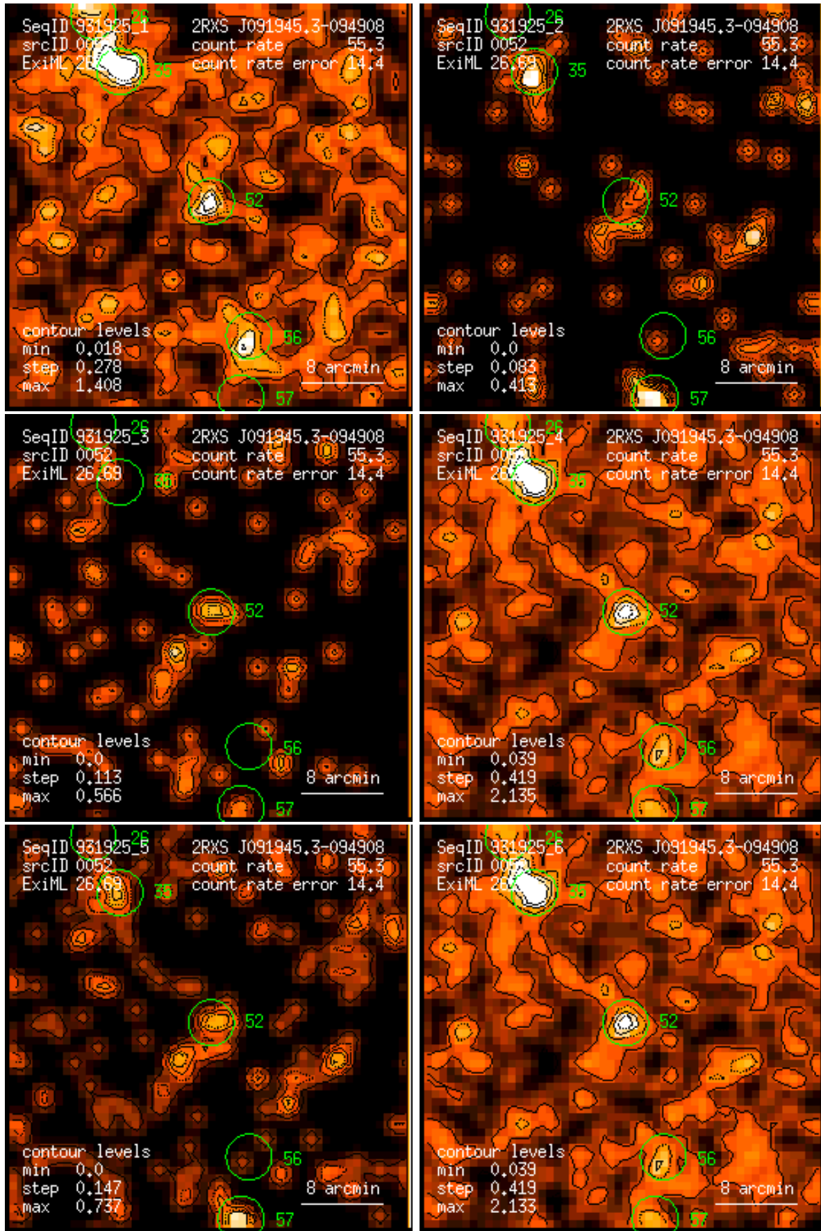
Figure 52: RASS 931925: detection 0052: band rate images, Gaussian filter: (1) PSPC channels 11 – 41, (2) 52 – 90, (3) 91 – 201, (4) 11 – 235, (5) 52 – 201, (6) 11 – 201. Broad band rates in counts/ks. Band rate contour levels in counts/ks/arcmin 2 .
