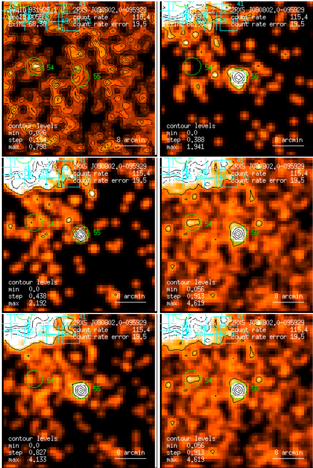
Figure 55: RASS 931925: detection 0055: band rate images, Gaussian filter: (1) PSPC channels 11 – 41, (2) 52 – 90, (3) 91 – 201, (4) 11 – 235, (5) 52 – 201, (6) 11 – 201. Broad band rates in counts/ks. Band rate contour levels in counts/ks/arcmin 2 .
