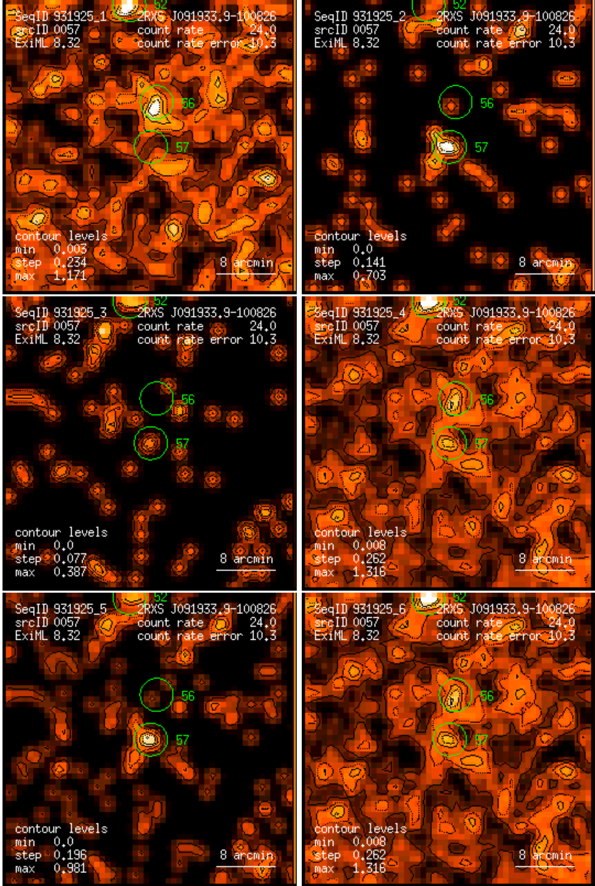
Figure 57: RASS 931925: detection 0057: band rate images, Gaussian filter: (1) PSPC channels 11 – 41, (2) 52 – 90, (3) 91 – 201, (4) 11 – 235, (5) 52 – 201, (6) 11 – 201. Broad band rates in counts/ks. Band rate contour levels in counts/ks/arcmin 2 .
