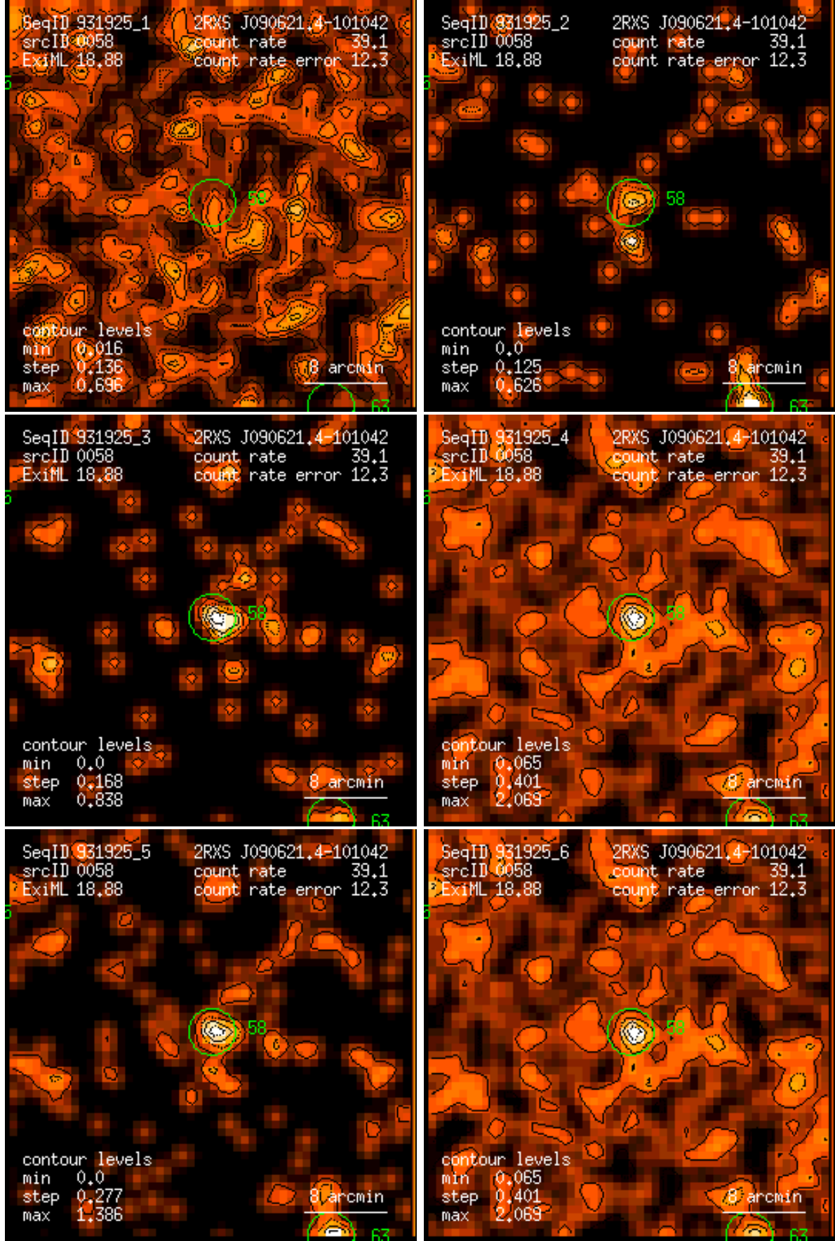
Figure 58: RASS 931925: detection 0058: band rate images, Gaussian filter: (1) PSPC channels 11 – 41, (2) 52 – 90, (3) 91 – 201, (4) 11 – 235, (5) 52 – 201, (6) 11 – 201. Broad band rates in counts/ks. Band rate contour levels in counts/ks/arcmin 2 .
