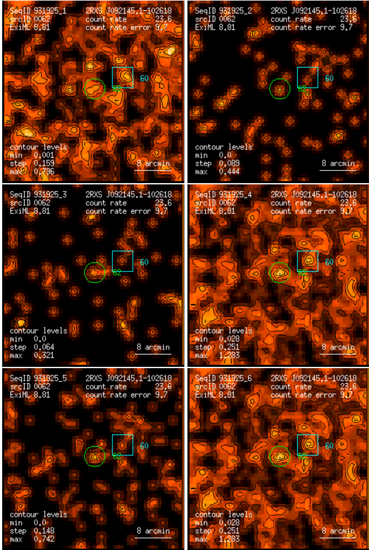
Figure 62: RASS 931925: detection 0062: band rate images, Gaussian filter: (1) PSPC channels 11 – 41, (2) 52 – 90, (3) 91 – 201, (4) 11 – 235, (5) 52 – 201, (6) 11 – 201. Broad band rates in counts/ks. Band rate contour levels in counts/ks/arcmin 2 .
