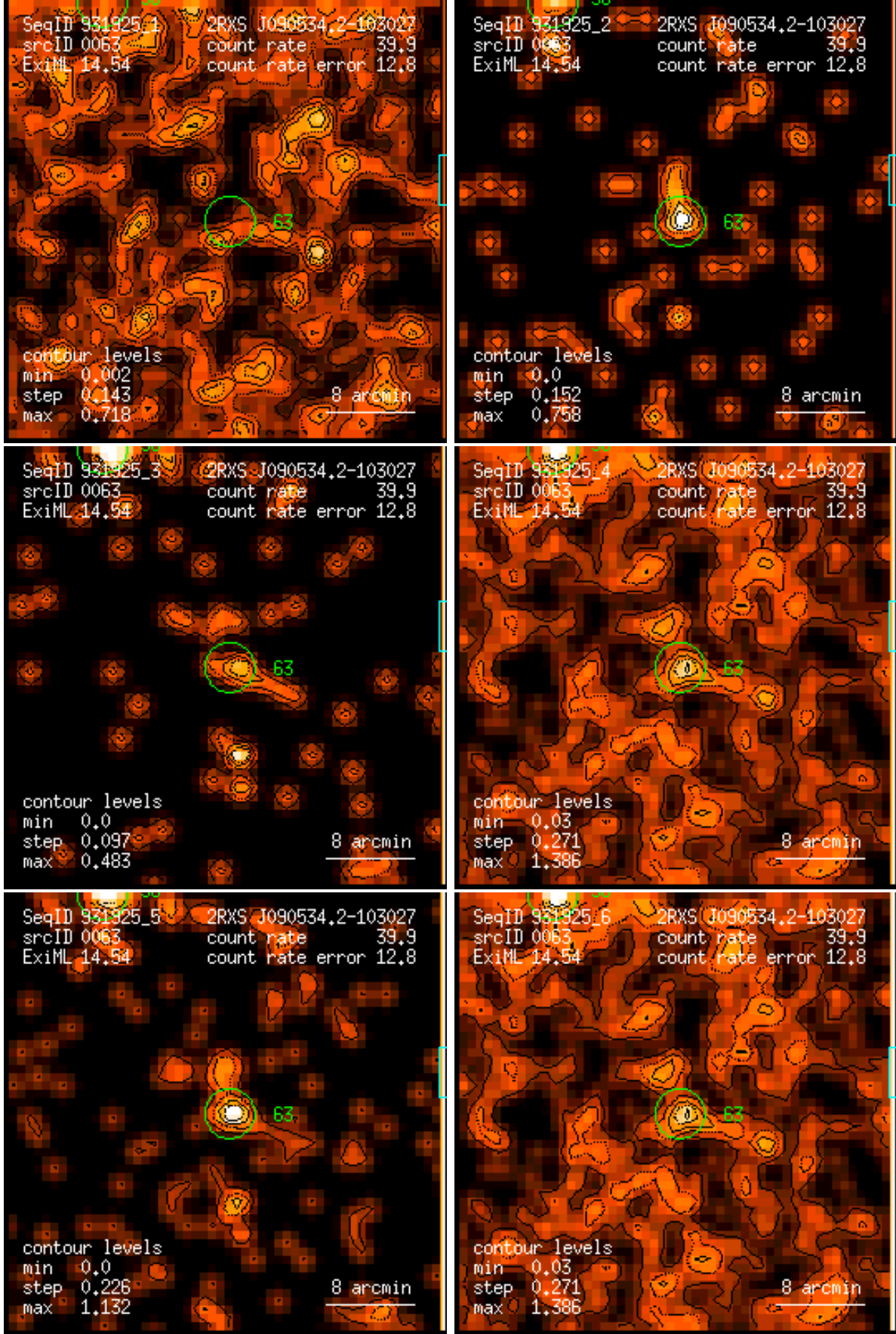
Figure 63: RASS 931925: detection 0063: band rate images, Gaussian filter: (1) PSPC channels 11 – 41, (2) 52 – 90, (3) 91 – 201, (4) 11 – 235, (5) 52 – 201, (6) 11 – 201. Broad band rates in counts/ks. Band rate contour levels in counts/ks/arcmin 2 .
