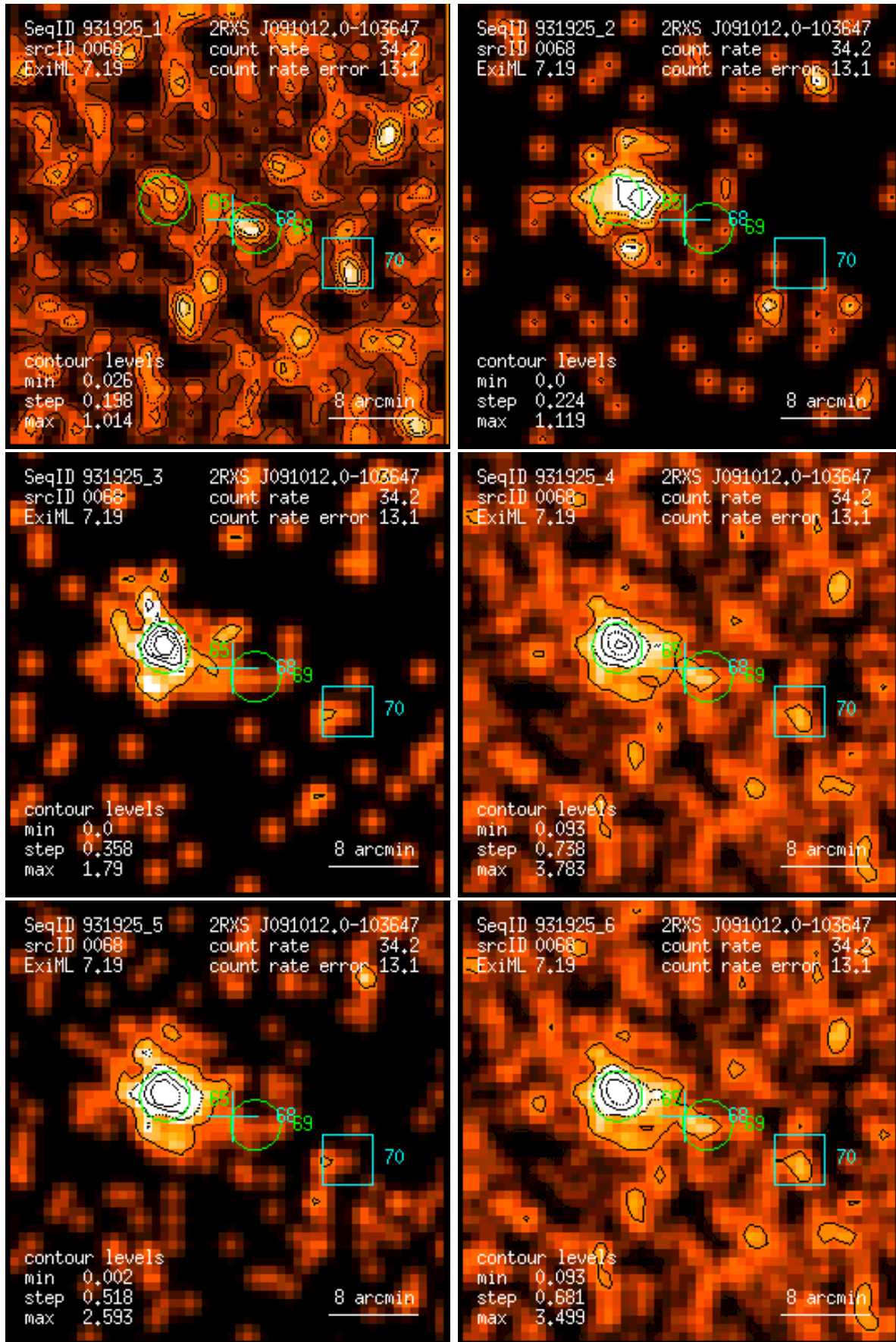
Figure 68: RASS 931925: detection 0068: band rate images, Gaussian filter: (1) PSPC channels 11 – 41, (2) 52 – 90, (3) 91 – 201, (4) 11 – 235, (5) 52 – 201, (6) 11 – 201. Broad band rates in counts/ks. Band rate contour levels in counts/ks/arcmin 2 .
