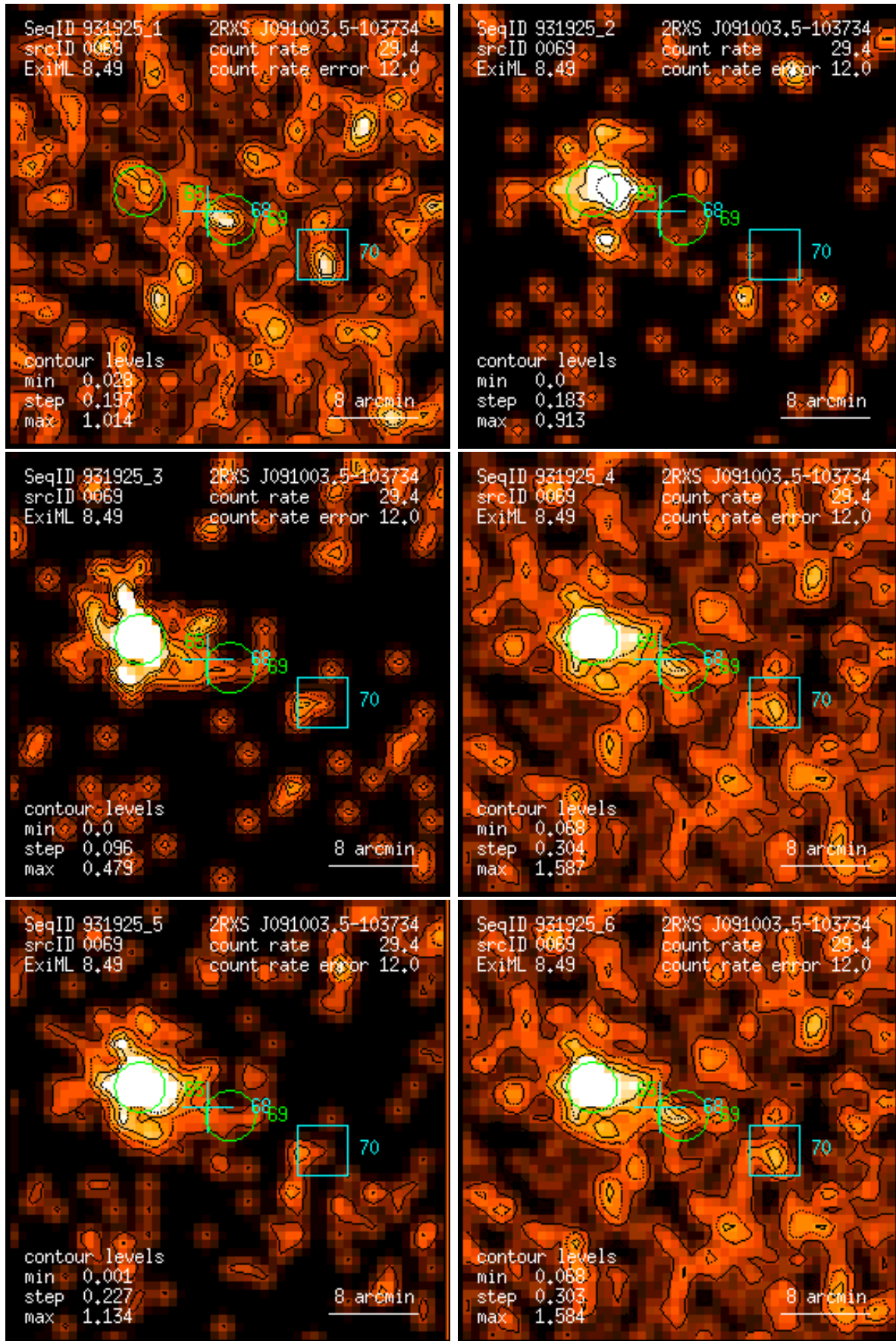
Figure 69: RASS 931925: detection 0069: band rate images, Gaussian filter: (1) PSPC channels 11 – 41, (2) 52 – 90, (3) 91 – 201, (4) 11 – 235, (5) 52 – 201, (6) 11 – 201. Broad band rates in counts/ks. Band rate contour levels in counts/ks/arcmin 2 .
