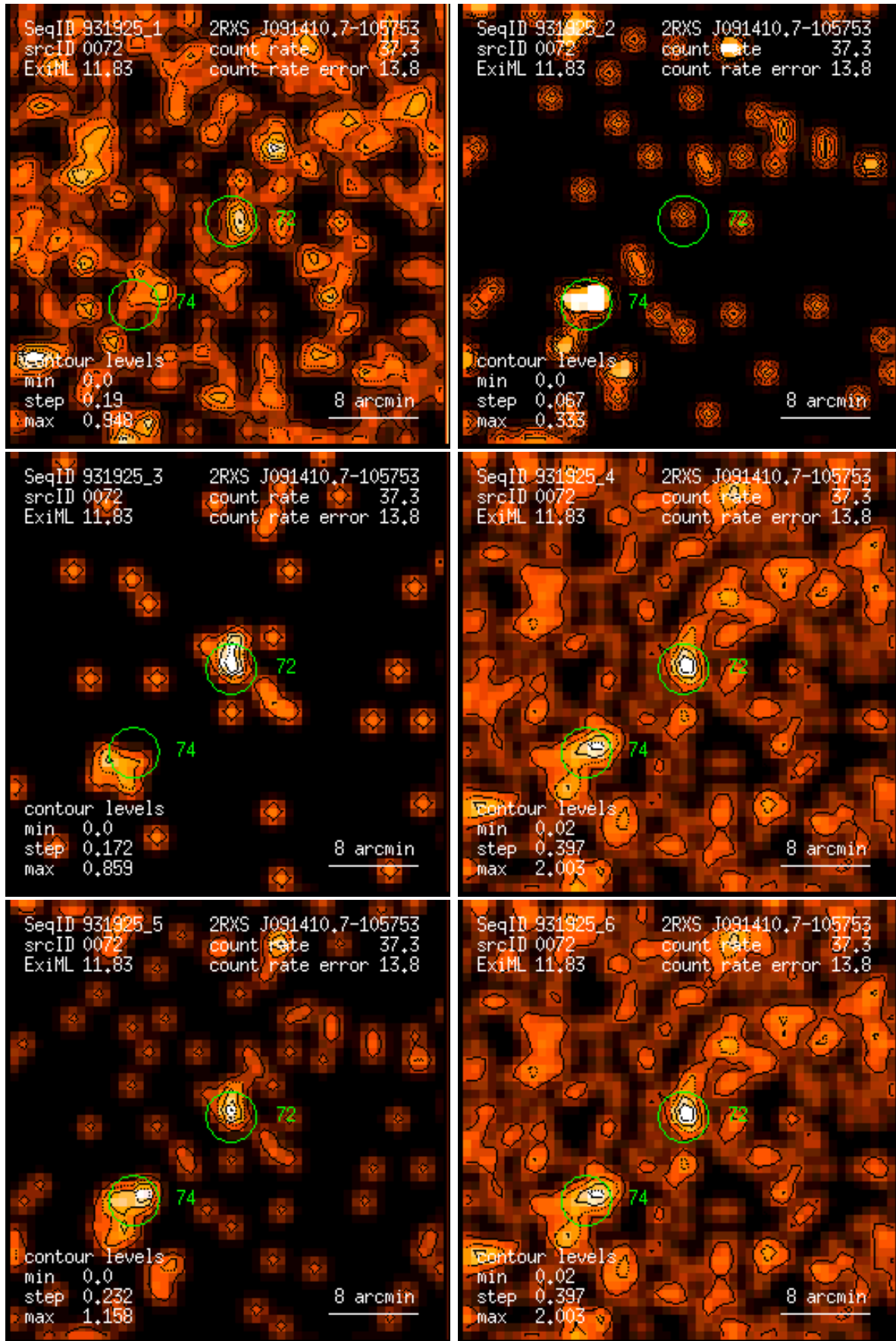
Figure 72: RASS 931925: detection 0072: band rate images, Gaussian filter: (1) PSPC channels 11 – 41, (2) 52 – 90, (3) 91 – 201, (4) 11 – 235, (5) 52 – 201, (6) 11 – 201. Broad band rates in counts/ks. Band rate contour levels in counts/ks/arcmin 2 .
