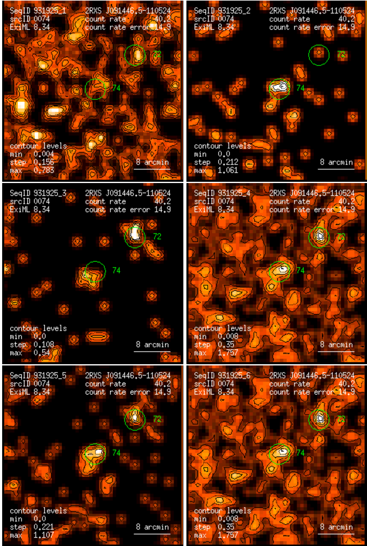
Figure 74: RASS 931925: detection 0074: band rate images, Gaussian filter: (1) PSPC channels 11 – 41, (2) 52 – 90, (3) 91 – 201, (4) 11 – 235, (5) 52 – 201, (6) 11 – 201. Broad band rates in counts/ks. Band rate contour levels in counts/ks/arcmin 2 .
