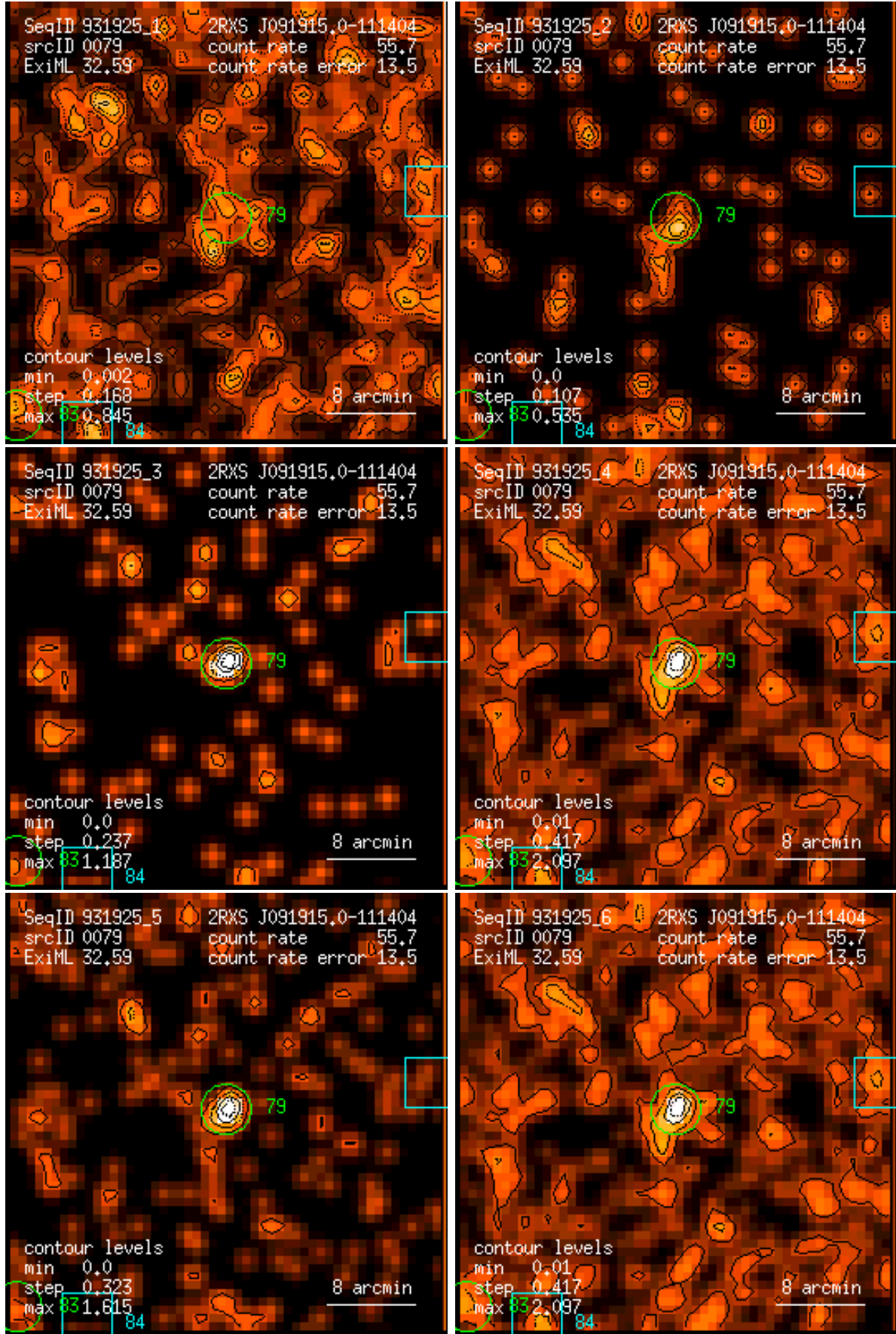
Figure 79: RASS 931925: detection 0079: band rate images, Gaussian filter: (1) PSPC channels 11 – 41, (2) 52 – 90, (3) 91 – 201, (4) 11 – 235, (5) 52 – 201, (6) 11 – 201. Broad band rates in counts/ks. Band rate contour levels in counts/ks/arcmin 2 .
