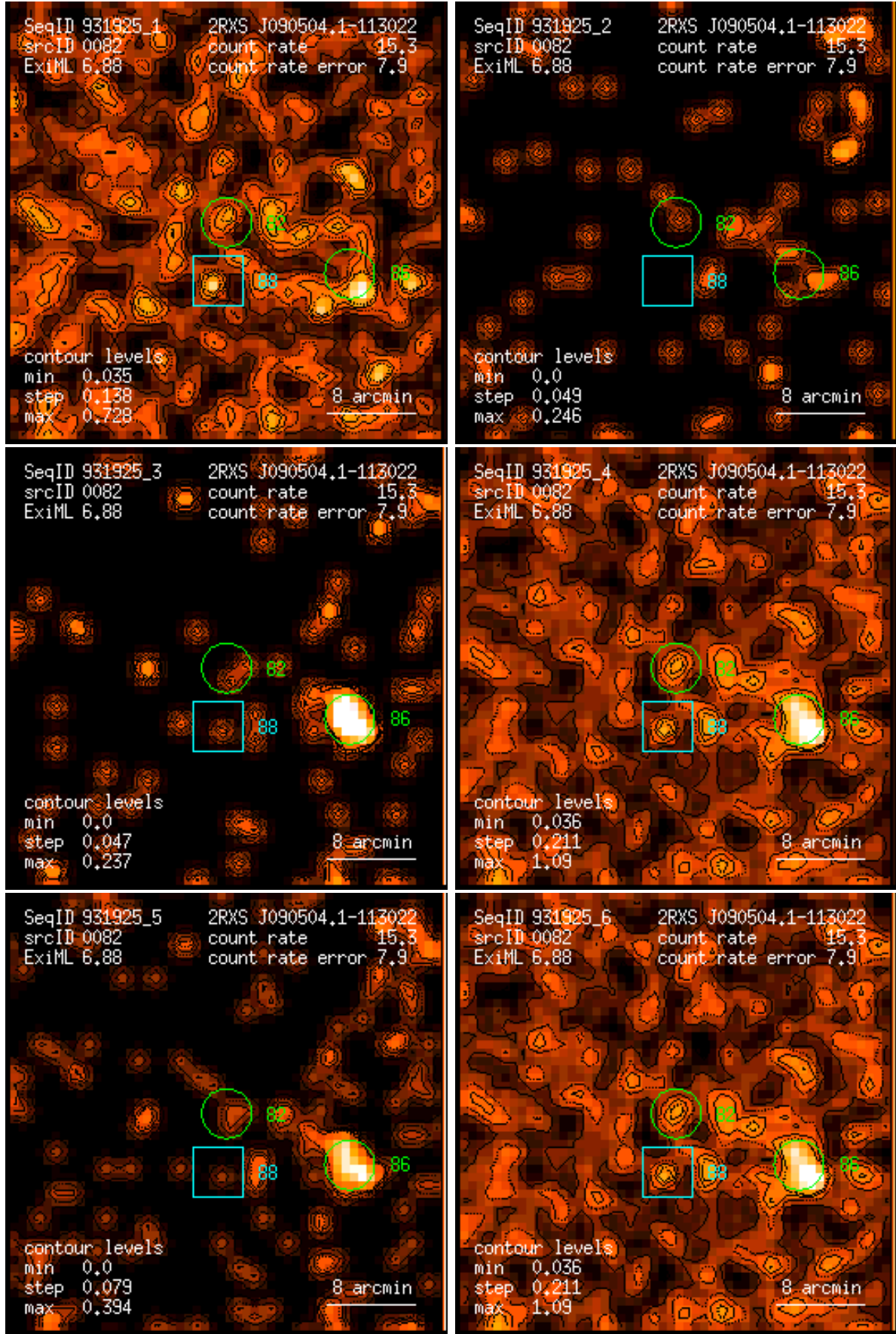
Figure 82: RASS 931925: detection 0082: band rate images, Gaussian filter: (1) PSPC channels 11 – 41, (2) 52 – 90, (3) 91 – 201, (4) 11 – 235, (5) 52 – 201, (6) 11 – 201. Broad band rates in counts/ks. Band rate contour levels in counts/ks/arcmin 2 .
