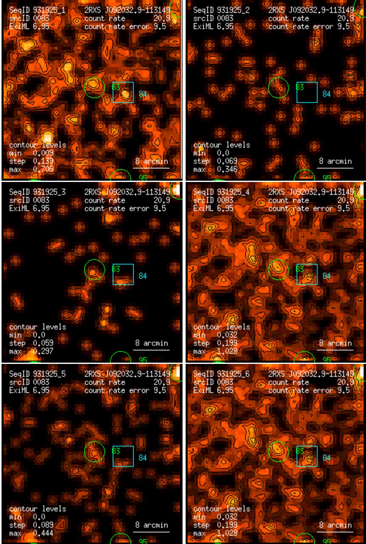
Figure 83: RASS 931925: detection 0083: band rate images, Gaussian filter: (1) PSPC channels 11 – 41, (2) 52 – 90, (3) 91 – 201, (4) 11 – 235, (5) 52 – 201, (6) 11 – 201. Broad band rates in counts/ks. Band rate contour levels in counts/ks/arcmin 2 .
