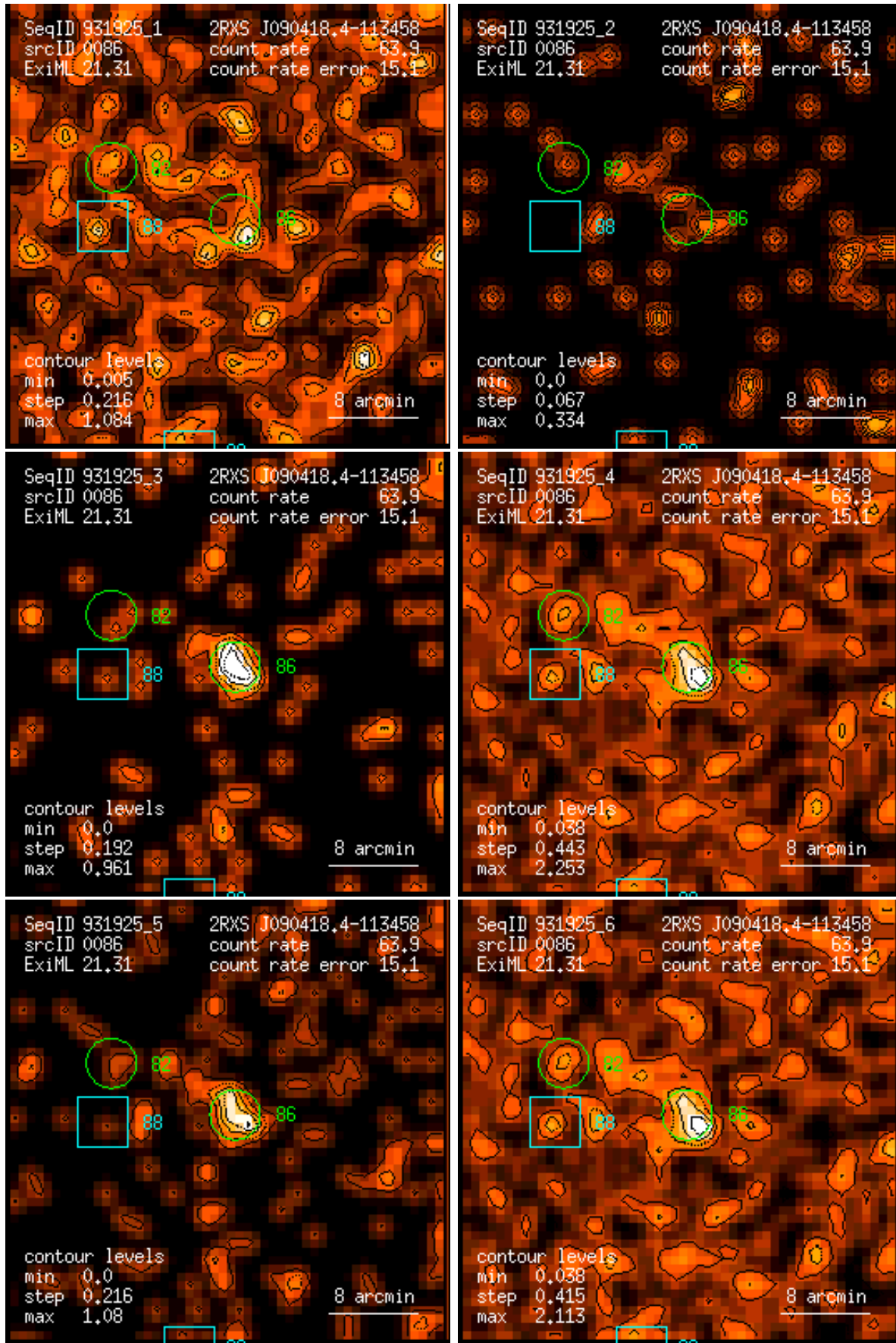
Figure 86: RASS 931925: detection 0086: band rate images, Gaussian filter: (1) PSPC channels 11 – 41, (2) 52 – 90, (3) 91 – 201, (4) 11 – 235, (5) 52 – 201, (6) 11 – 201. Broad band rates in counts/ks. Band rate contour levels in counts/ks/arcmin 2 .
