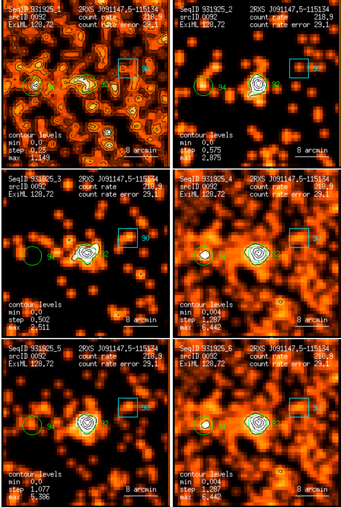
Figure 92: RASS 931925: detection 0092: band rate images, Gaussian filter: (1) PSPC channels 11 – 41, (2) 52 – 90, (3) 91 – 201, (4) 11 – 235, (5) 52 – 201, (6) 11 – 201. Broad band rates in counts/ks. Band rate contour levels in counts/ks/arcmin 2 .
