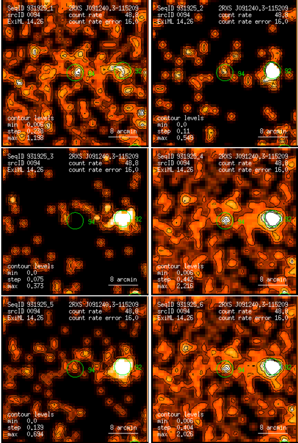
Figure 94: RASS 931925: detection 0094: band rate images, Gaussian filter: (1) PSPC channels 11 – 41, (2) 52 – 90, (3) 91 – 201, (4) 11 – 235, (5) 52 – 201, (6) 11 – 201. Broad band rates in counts/ks. Band rate contour levels in counts/ks/arcmin 2 .
