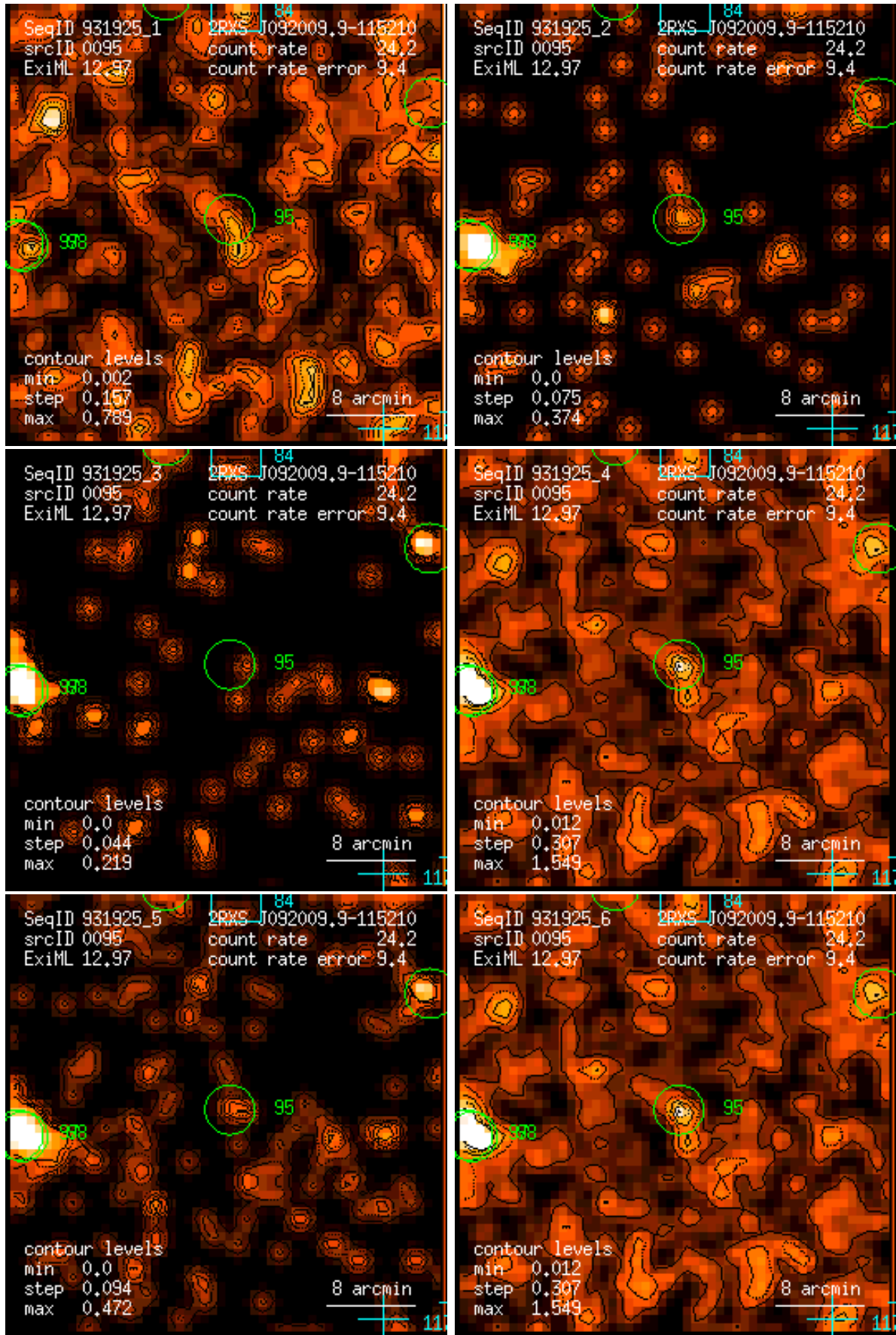
Figure 95: RASS 931925: detection 0095: band rate images, Gaussian filter: (1) PSPC channels 11 – 41, (2) 52 – 90, (3) 91 – 201, (4) 11 – 235, (5) 52 – 201, (6) 11 – 201. Broad band rates in counts/ks. Band rate contour levels in counts/ks/arcmin 2 .
