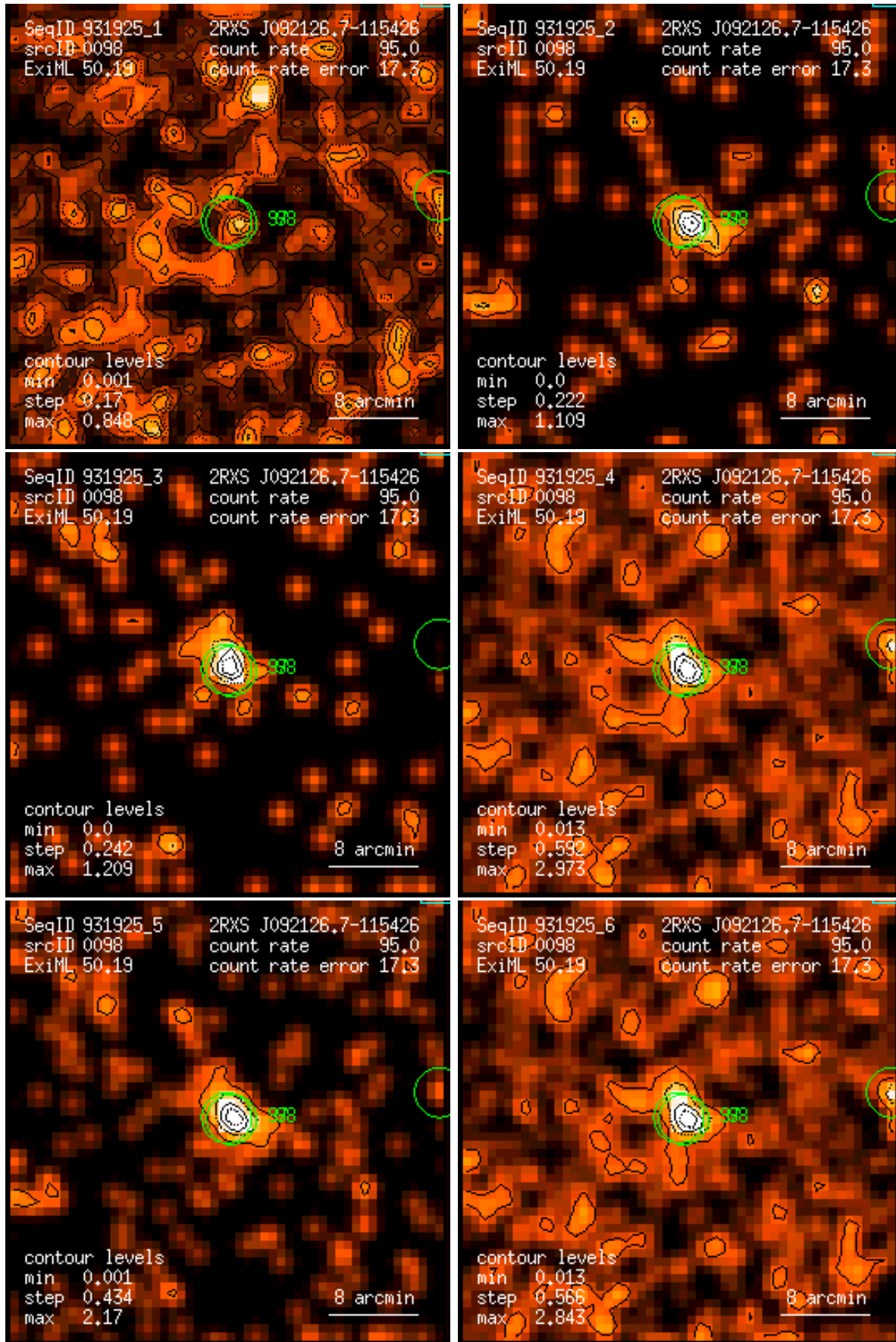
Figure 98: RASS 931925: detection 0098: band rate images, Gaussian filter: (1) PSPC channels 11 – 41, (2) 52 – 90, (3) 91 – 201, (4) 11 – 235, (5) 52 – 201, (6) 11 – 201. Broad band rates in counts/ks. Band rate contour levels in counts/ks/arcmin 2 .
