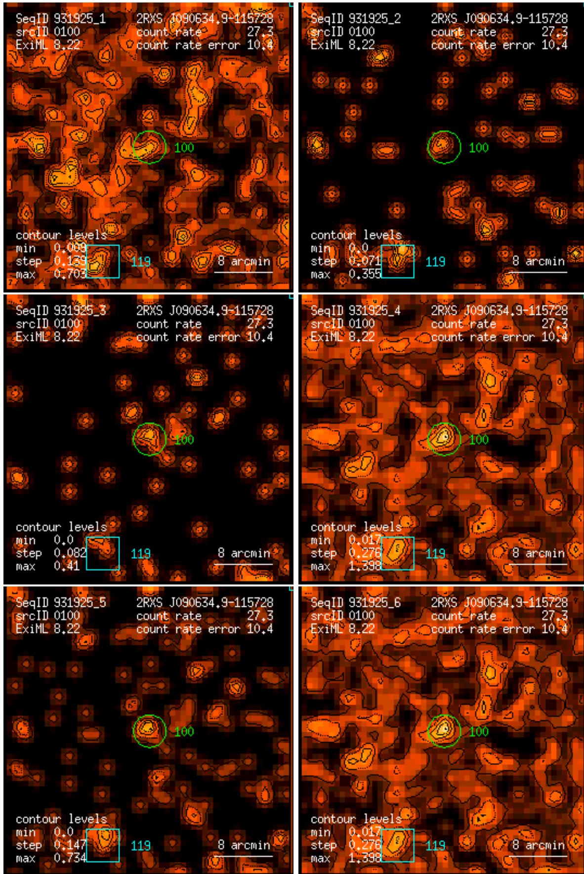
Figure 100: RASS 931925: detection 0100: band rate images, Gaussian filter: (1) PSPC channels 11 – 41, (2) 52 – 90, (3) 91 – 201, (4) 11 – 235, (5) 52 – 201, (6) 11 – 201. Broad band rates in counts/ks. Band rate contour levels in counts/ks/arcmin 2 .
