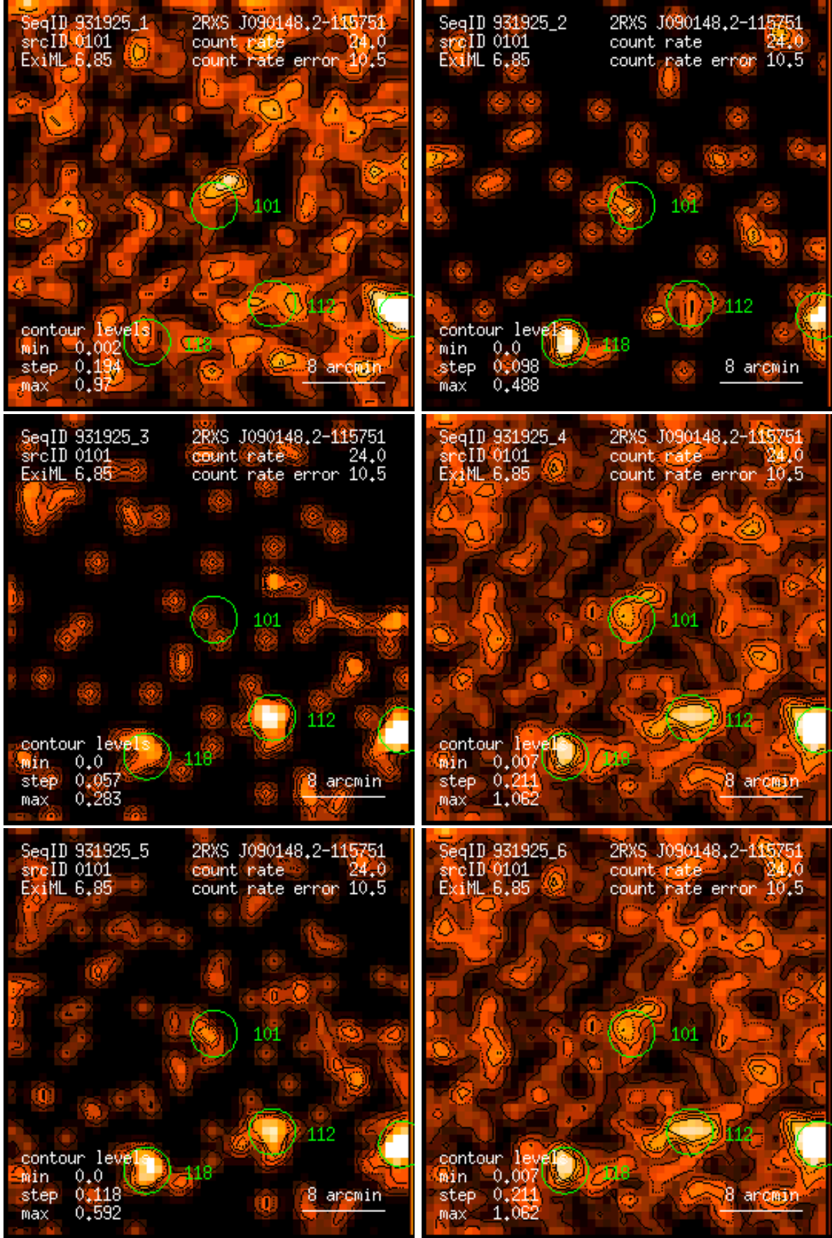
Figure 101: RASS 931925: detection 0101: band rate images, Gaussian filter: (1) PSPC channels 11 – 41, (2) 52 – 90, (3) 91 – 201, (4) 11 – 235, (5) 52 – 201, (6) 11 – 201. Broad band rates in counts/ks. Band rate contour levels in counts/ks/arcmin 2 .
