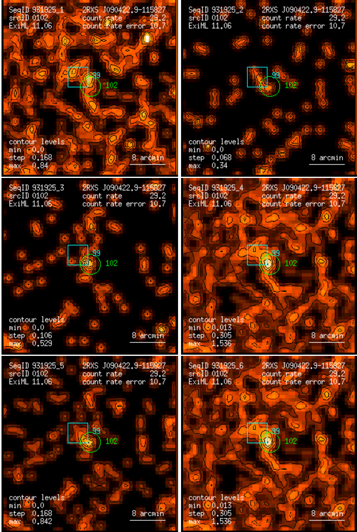
Figure 102: RASS 931925: detection 0102: band rate images, Gaussian filter: (1) PSPC channels 11 – 41, (2) 52 – 90, (3) 91 – 201, (4) 11 – 235, (5) 52 – 201, (6) 11 – 201. Broad band rates in counts/ks. Band rate contour levels in counts/ks/arcmin 2 .
