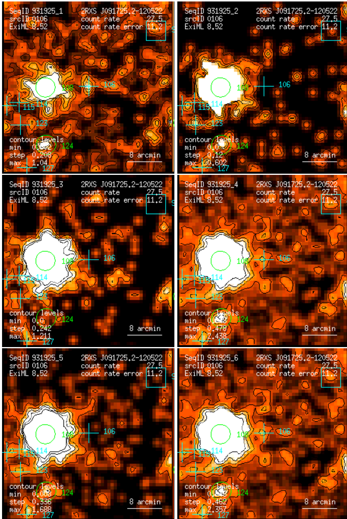
Figure 106: RASS 931925: detection 0106: band rate images, Gaussian filter: (1) PSPC channels 11 – 41, (2) 52 – 90, (3) 91 – 201, (4) 11 – 235, (5) 52 – 201, (6) 11 – 201. Broad band rates in counts/ks. Band rate contour levels in counts/ks/arcmin 2 .
