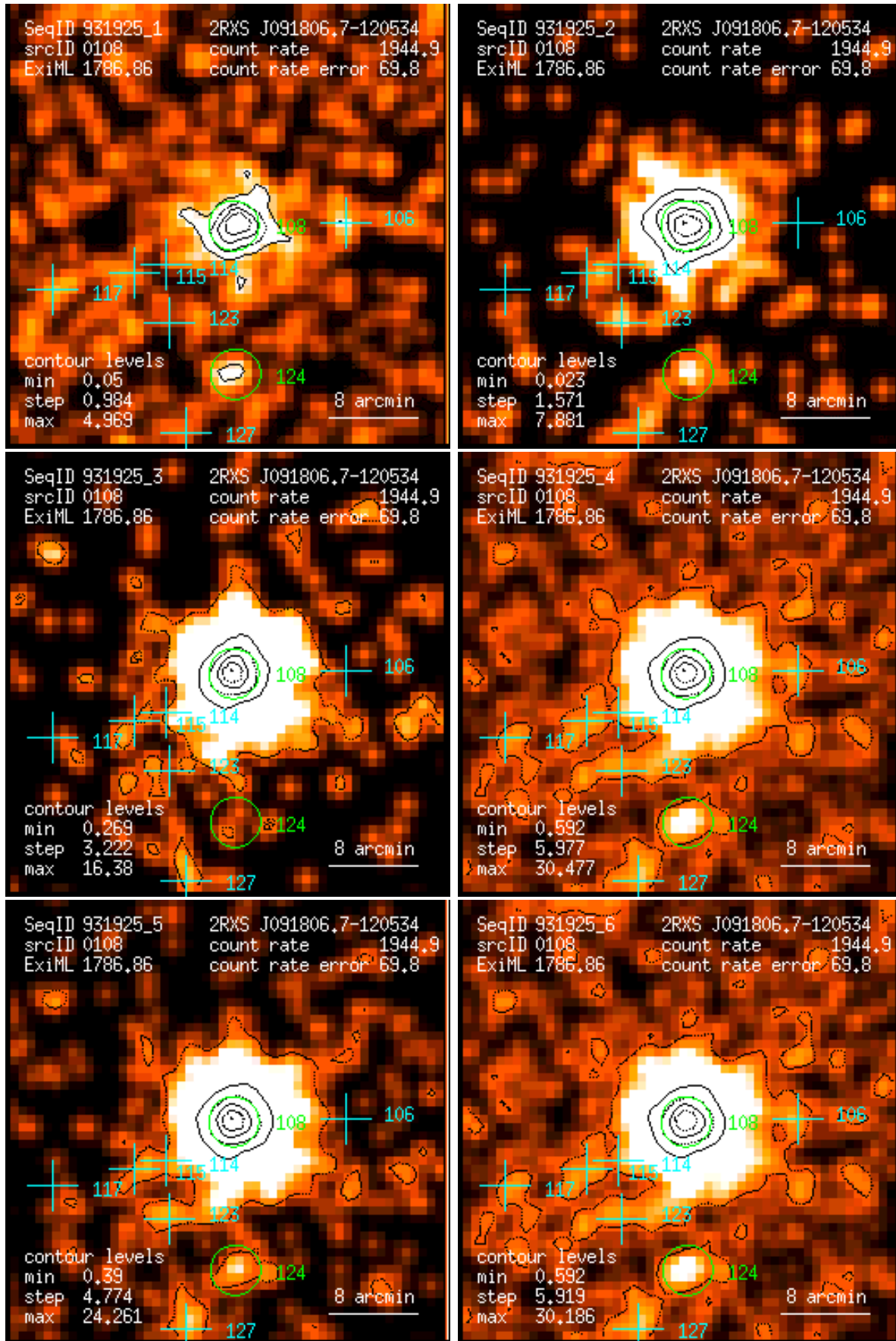
Figure 108: RASS 931925: detection 0108: band rate images, Gaussian filter: (1) PSPC channels 11 – 41, (2) 52 – 90, (3) 91 – 201, (4) 11 – 235, (5) 52 – 201, (6) 11 – 201. Broad band rates in counts/ks. Band rate contour levels in counts/ks/arcmin 2 .
