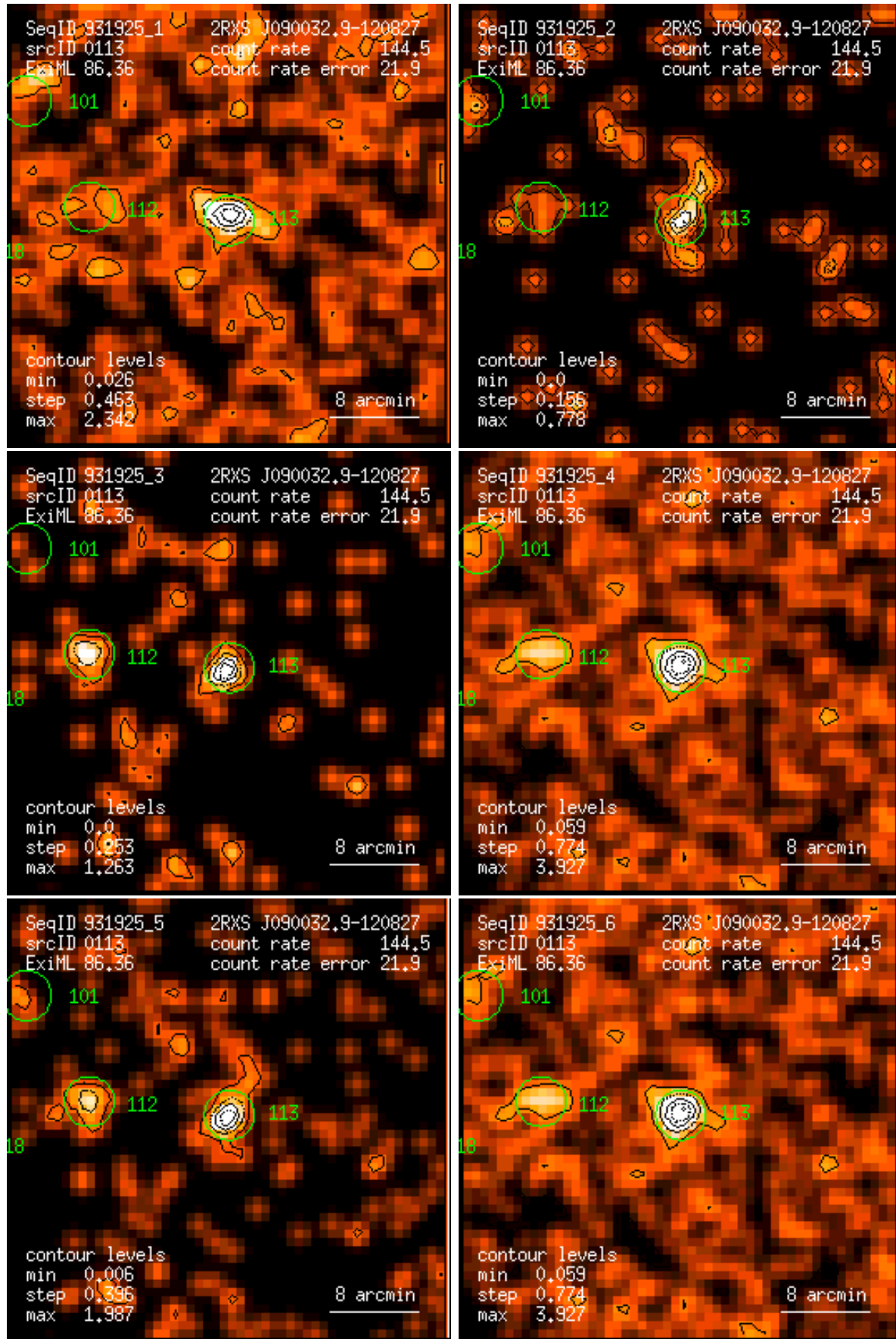
Figure 113: RASS 931925: detection 0113: band rate images, Gaussian filter: (1) PSPC channels 11 – 41, (2) 52 – 90, (3) 91 – 201, (4) 11 – 235, (5) 52 – 201, (6) 11 – 201. Broad band rates in counts/ks. Band rate contour levels in counts/ks/arcmin 2 .
