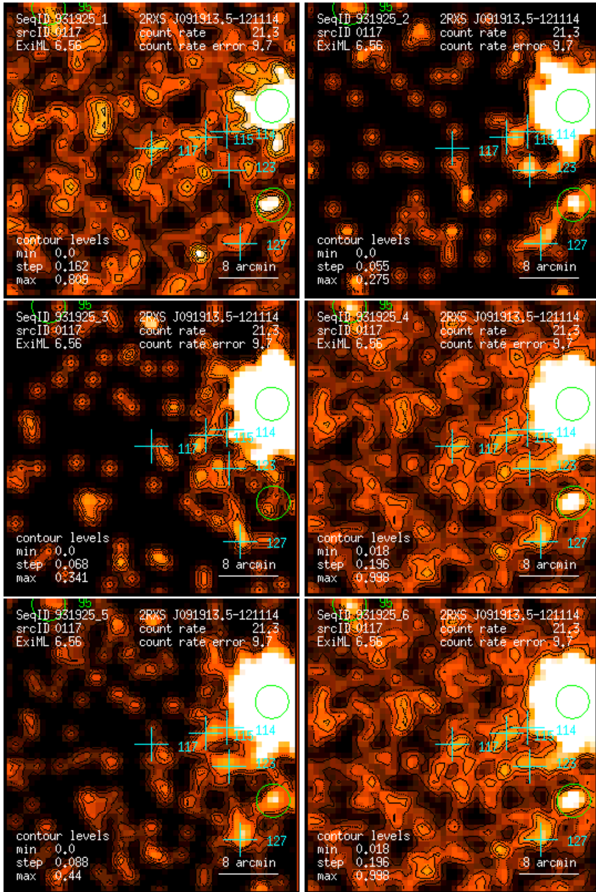
Figure 117: RASS 931925: detection 0117: band rate images, Gaussian filter: (1) PSPC channels 11 – 41, (2) 52 – 90, (3) 91 – 201, (4) 11 – 235, (5) 52 – 201, (6) 11 – 201. Broad band rates in counts/ks. Band rate contour levels in counts/ks/arcmin 2 .
