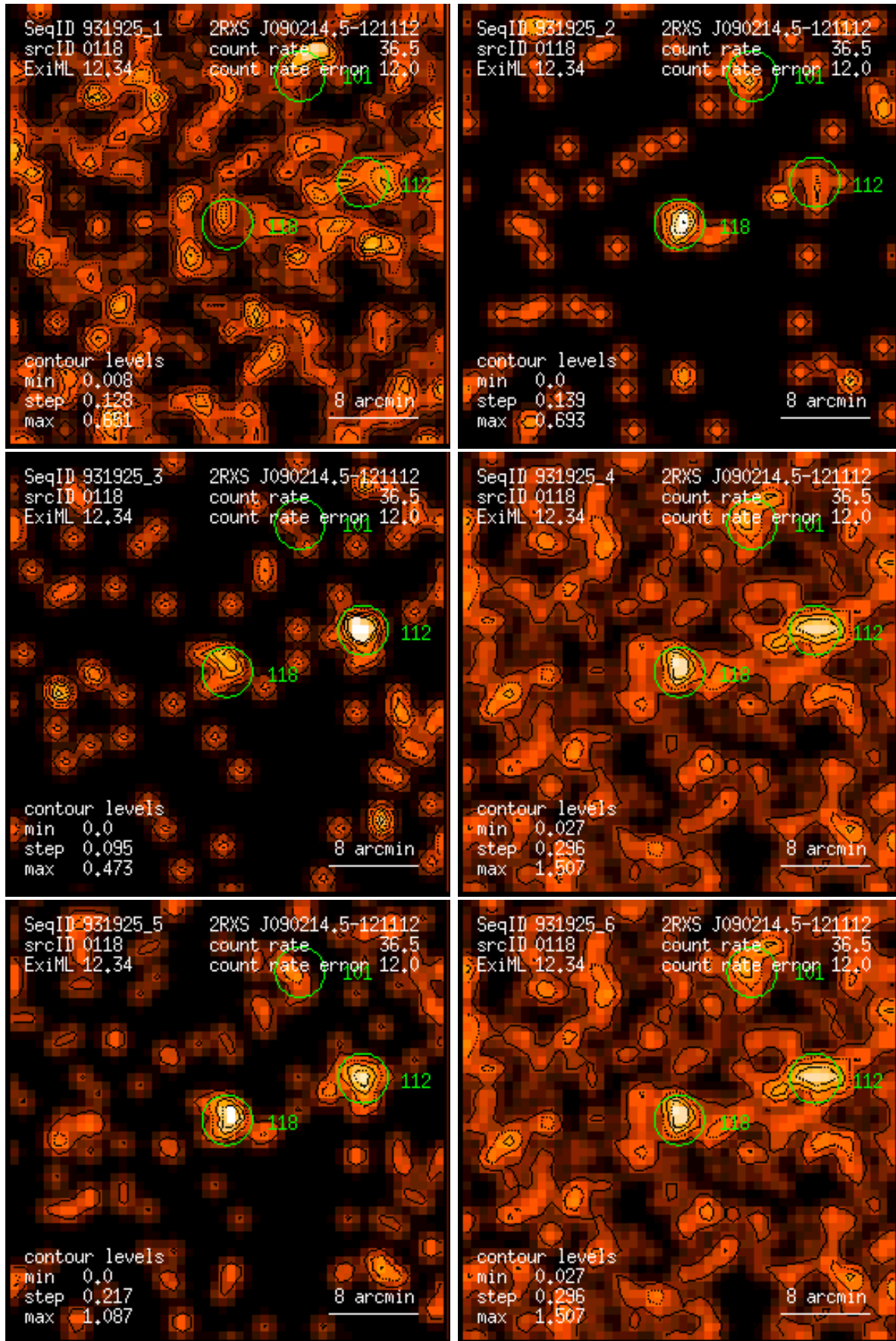
Figure 118: RASS 931925: detection 0118: band rate images, Gaussian filter: (1) PSPC channels 11 – 41, (2) 52 – 90, (3) 91 – 201, (4) 11 – 235, (5) 52 – 201, (6) 11 – 201. Broad band rates in counts/ks. Band rate contour levels in counts/ks/arcmin 2 .
