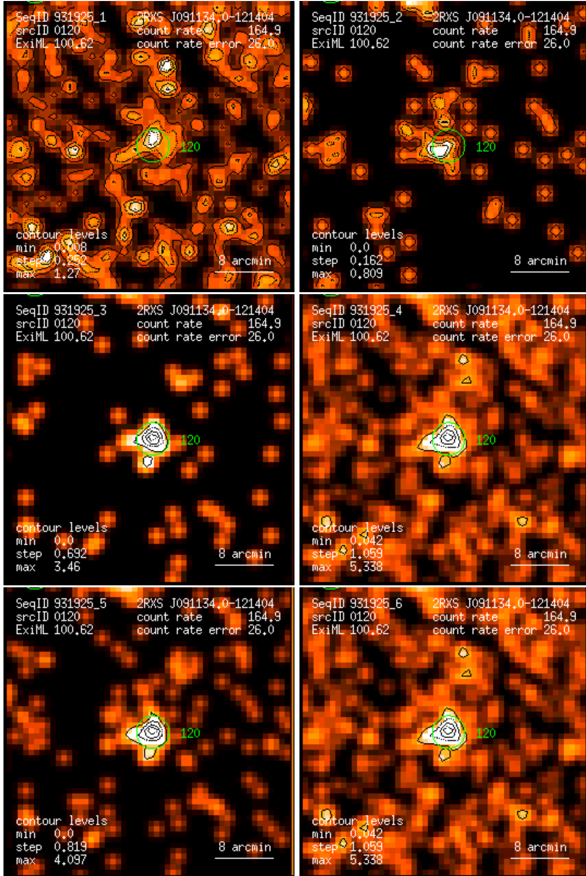
Figure 120: RASS 931925: detection 0120: band rate images, Gaussian filter: (1) PSPC channels 11 – 41, (2) 52 – 90, (3) 91 – 201, (4) 11 – 235, (5) 52 – 201, (6) 11 – 201. Broad band rates in counts/ks. Band rate contour levels in counts/ks/arcmin 2 .
