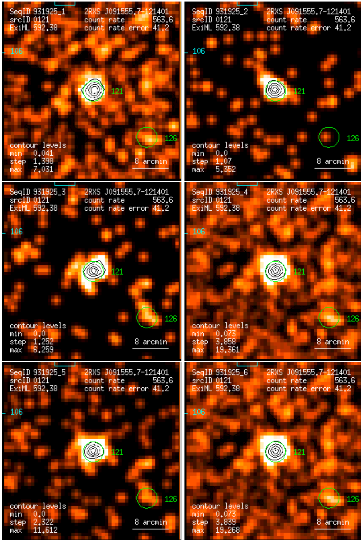
Figure 121: RASS 931925: detection 0121: band rate images, Gaussian filter: (1) PSPC channels 11 – 41, (2) 52 – 90, (3) 91 – 201, (4) 11 – 235, (5) 52 – 201, (6) 11 – 201. Broad band rates in counts/ks. Band rate contour levels in counts/ks/arcmin 2 .
