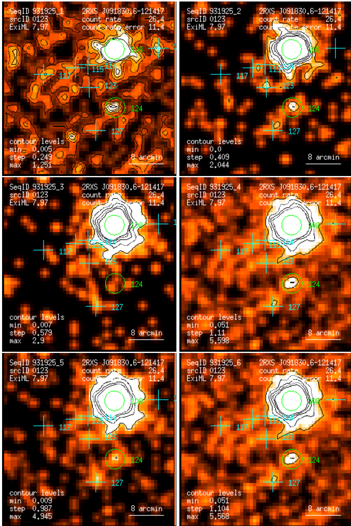
Figure 123: RASS 931925: detection 0123: band rate images, Gaussian filter: (1) PSPC channels 11 – 41, (2) 52 – 90, (3) 91 – 201, (4) 11 – 235, (5) 52 – 201, (6) 11 – 201. Broad band rates in counts/ks. Band rate contour levels in counts/ks/arcmin 2 .
