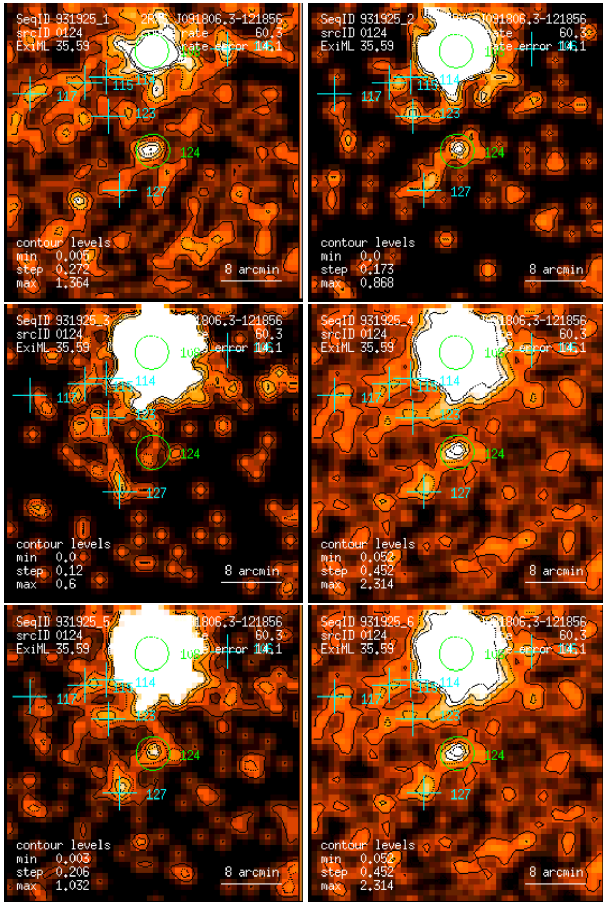
Figure 124: RASS 931925: detection 0124: band rate images, Gaussian filter: (1) PSPC channels 11 – 41, (2) 52 – 90, (3) 91 – 201, (4) 11 – 235, (5) 52 – 201, (6) 11 – 201. Broad band rates in counts/ks. Band rate contour levels in counts/ks/arcmin 2 .
