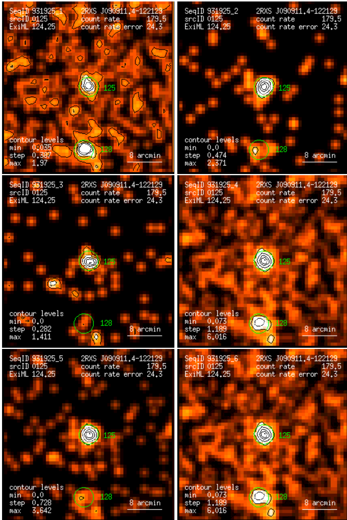
Figure 125: RASS 931925: detection 0125: band rate images, Gaussian filter: (1) PSPC channels 11 – 41, (2) 52 – 90, (3) 91 – 201, (4) 11 – 235, (5) 52 – 201, (6) 11 – 201. Broad band rates in counts/ks. Band rate contour levels in counts/ks/arcmin 2 .
