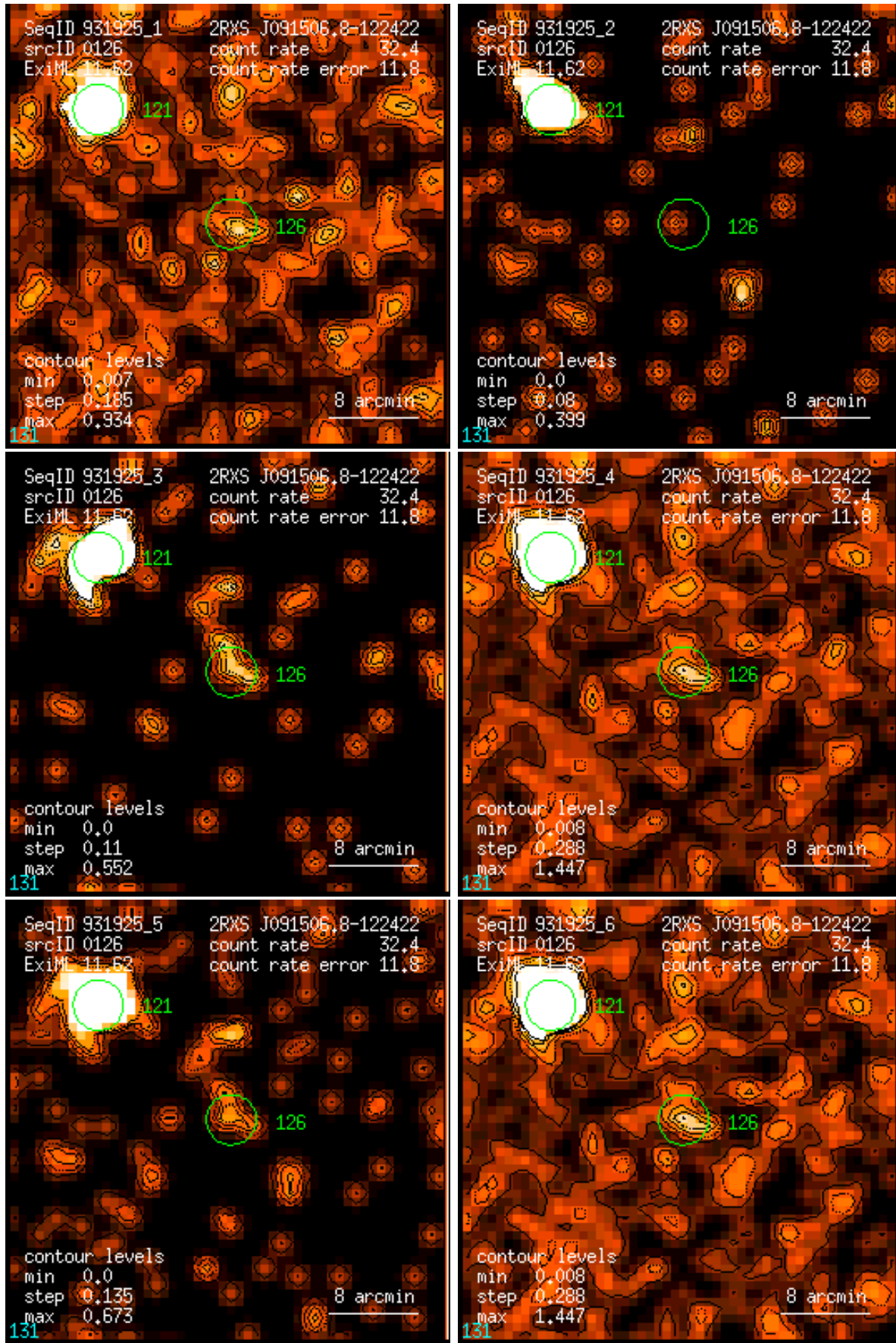
Figure 126: RASS 931925: detection 0126: band rate images, Gaussian filter: (1) PSPC channels 11 – 41, (2) 52 – 90, (3) 91 – 201, (4) 11 – 235, (5) 52 – 201, (6) 11 – 201. Broad band rates in counts/ks. Band rate contour levels in counts/ks/arcmin 2 .
