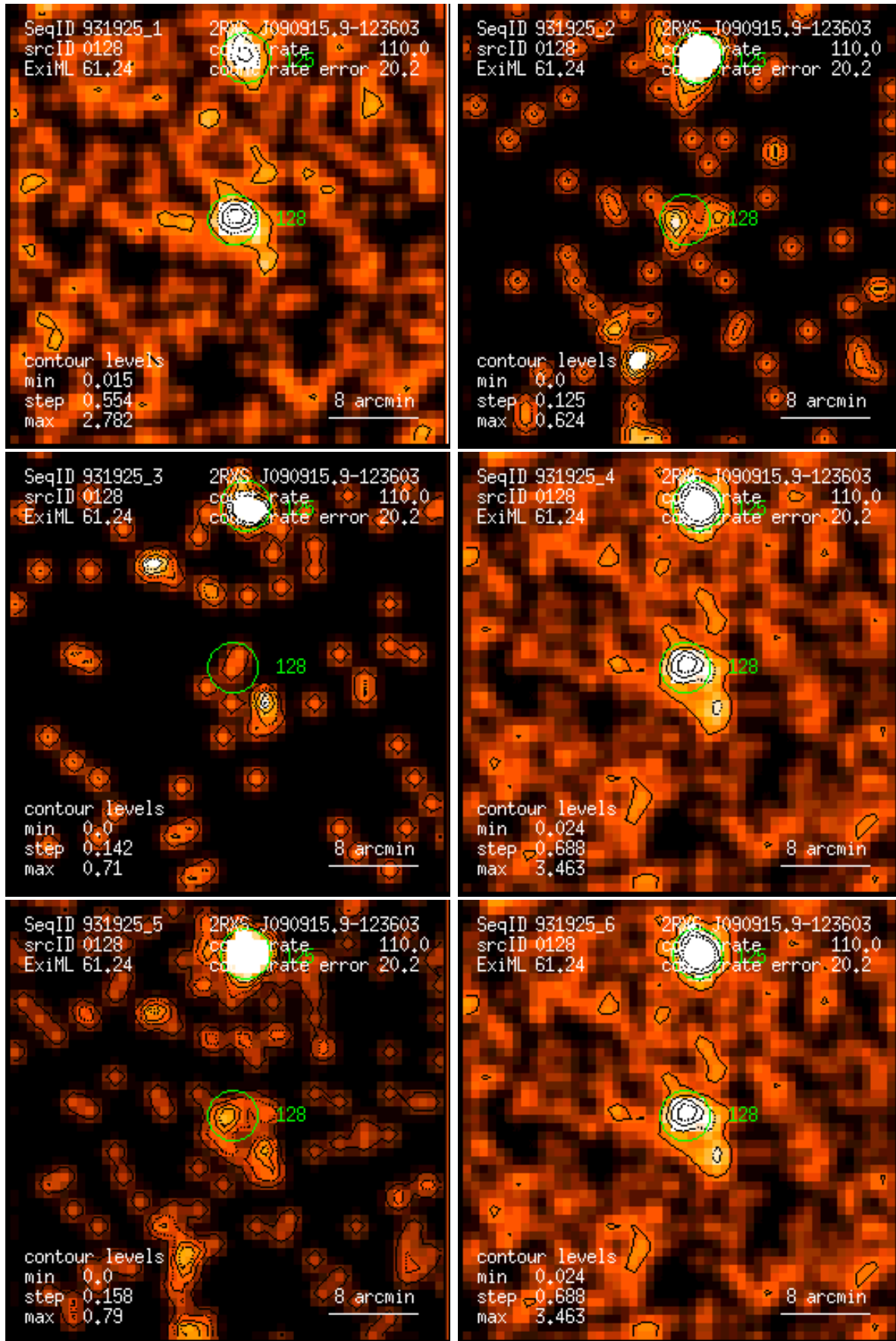
Figure 128: RASS 931925: detection 0128: band rate images, Gaussian filter: (1) PSPC channels 11 – 41, (2) 52 – 90, (3) 91 – 201, (4) 11 – 235, (5) 52 – 201, (6) 11 – 201. Broad band rates in counts/ks. Band rate contour levels in counts/ks/arcmin 2 .
