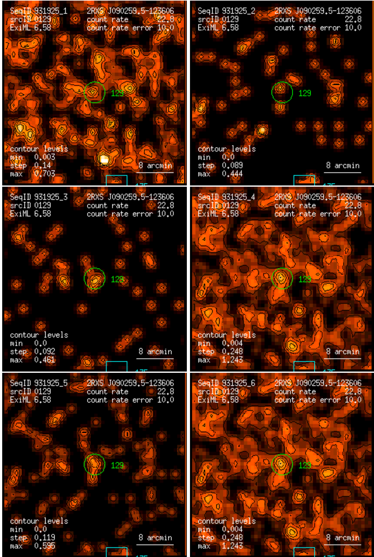
Figure 129: RASS 931925: detection 0129: band rate images, Gaussian filter: (1) PSPC channels 11 – 41, (2) 52 – 90, (3) 91 – 201, (4) 11 – 235, (5) 52 – 201, (6) 11 – 201. Broad band rates in counts/ks. Band rate contour levels in counts/ks/arcmin 2 .
