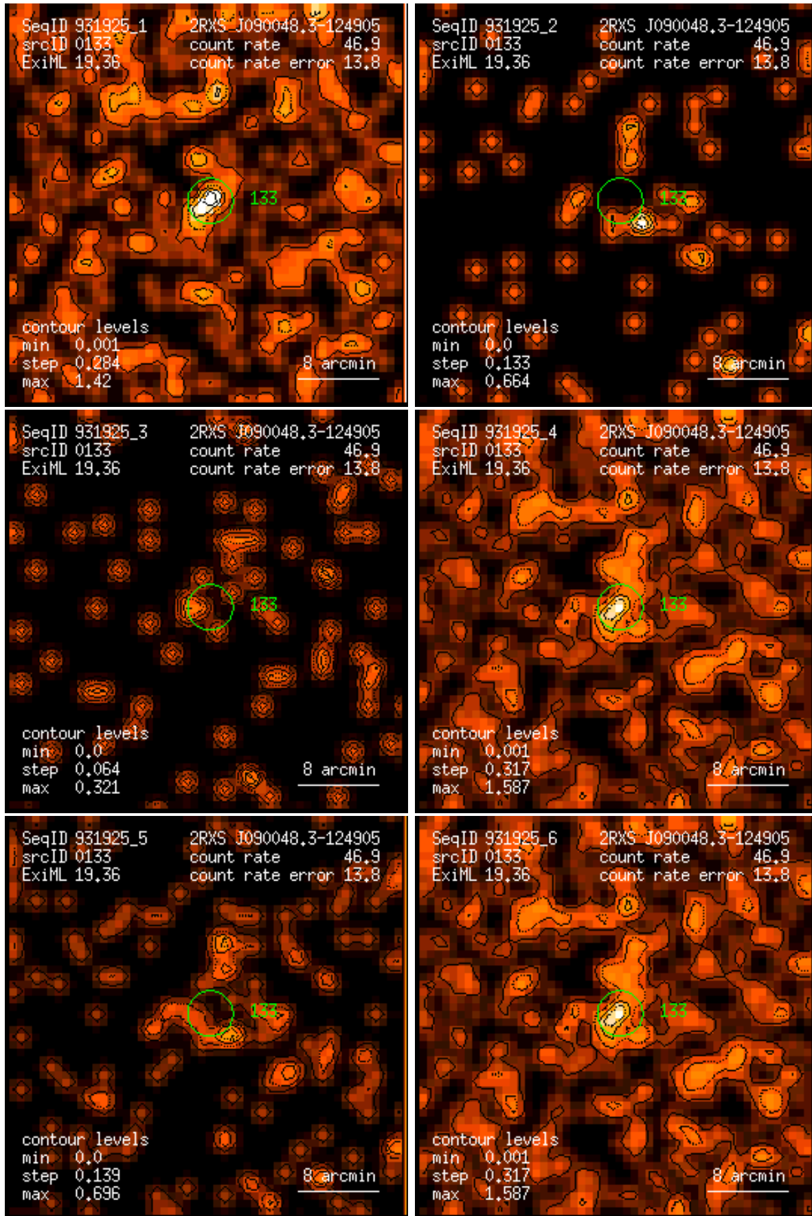
Figure 133: RASS 931925: detection 0133: band rate images, Gaussian filter: (1) PSPC channels 11 – 41, (2) 52 – 90, (3) 91 – 201, (4) 11 – 235, (5) 52 – 201, (6) 11 – 201. Broad band rates in counts/ks. Band rate contour levels in counts/ks/arcmin 2 .
