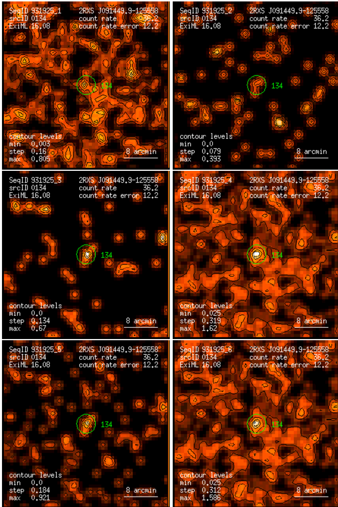
Figure 134: RASS 931925: detection 0134: band rate images, Gaussian filter: (1) PSPC channels 11 – 41, (2) 52 – 90, (3) 91 – 201, (4) 11 – 235, (5) 52 – 201, (6) 11 – 201. Broad band rates in counts/ks. Band rate contour levels in counts/ks/arcmin 2 .
